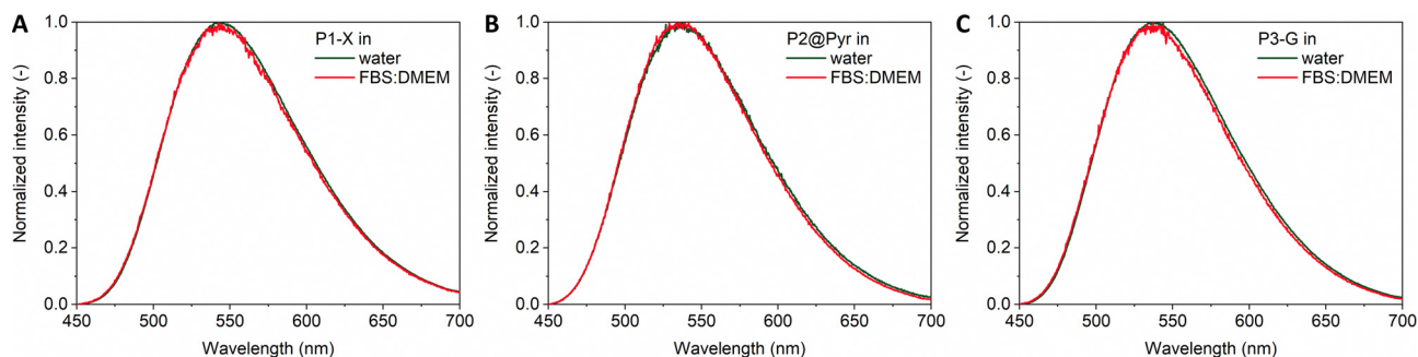
Fig. 2 Normalized fluorescence spectra of (A) P1-X , (B) P2@Pyr , and (C) P3-G in water and 10 : 90 vol% FBS:DMEM ( c_{\text{pol}} = 3 \text{ mg mL}^{-1} , c_{\text{pyr}} , P1-X = 140 \mu\text{M} , c_{\text{pyr}} , P2@Pyr = 20 \mu\text{M} , c_{\text{pyr}} , P3-G = 150 \mu\text{M} , \lambda_{\text{ex}} = 405 \text{ nm} ).
