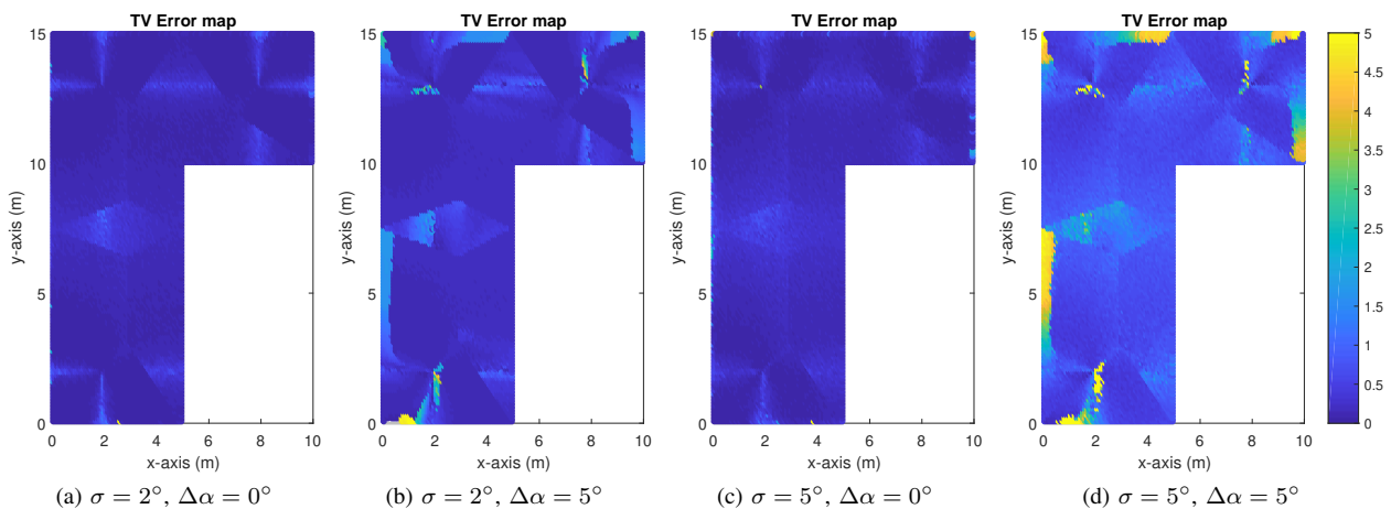
Figure 7. Median localization error maps for TV, for different values of \sigma and \Delta\alpha . N_{\text{AP}} = 3 .
