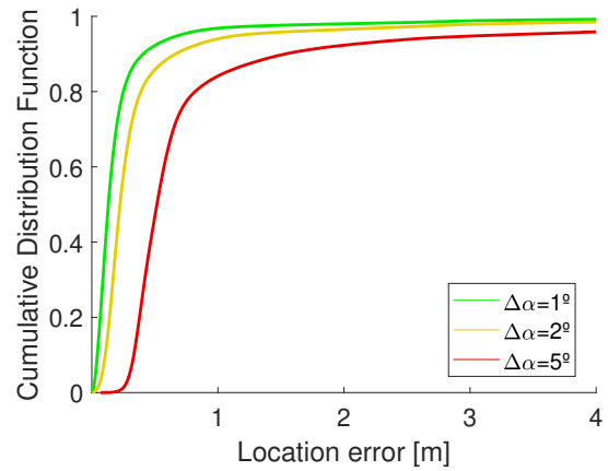
Figure 5. CDF of the localization error for TV as a function of the client’s compass bias, \Delta\alpha . N_{AP} = 3 , \sigma = 2^\circ .
