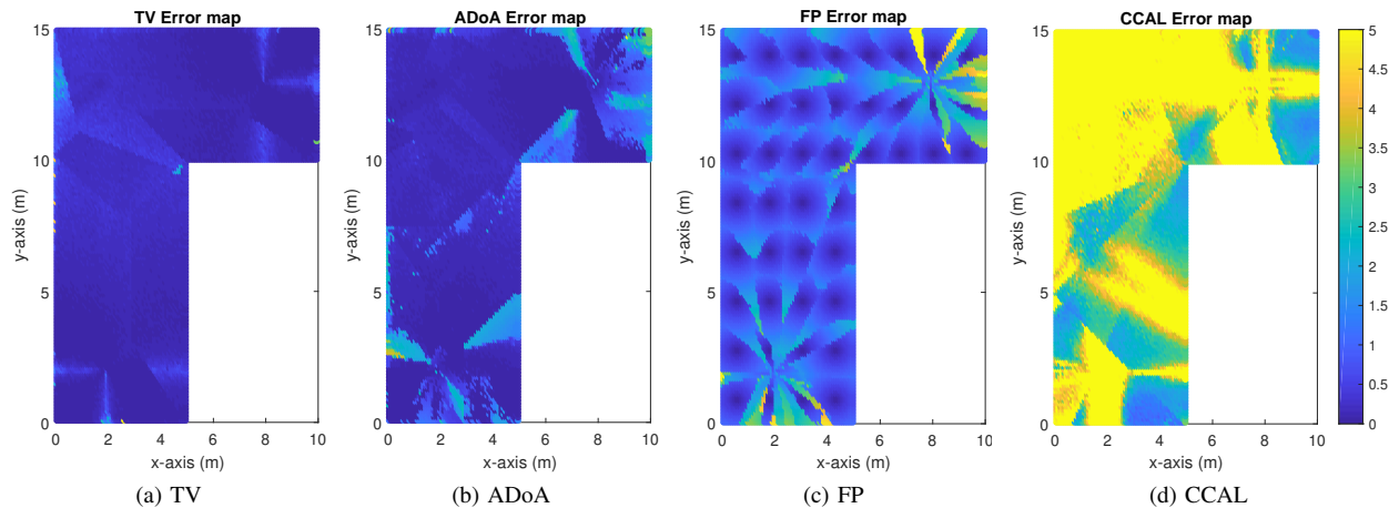
Figure 6. Median localization error maps for all methods, \sigma = 2^\circ , N_{\text{AP}} = 2 , \Delta\alpha = 0 .
