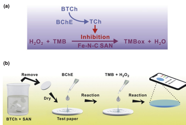
Figure 7 Application of single-atom nanozyme in the detection of BChE activity. (a) Illustration of the biosensing principle of BChE activity. BTCh: S-butylthiocholine iodide. (b) Illustration of the paper bioassay procedure for BChE activity. Reproduced with permission from Ref. [107], © Elsevier B.V. 2019.
