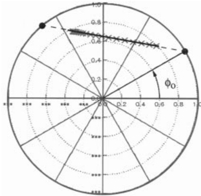
Fig. 6. Geometrical interpretation of polarimetric interferometry for the random volume over ground scattering model.
