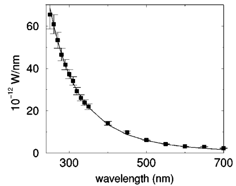
FIG. 5. Spectrum of single-bubble sonoluminescence, for water at 22 ^{\circ}\text{C} . The data points are redrawn from Fig. 1 of Hiller et al. (1992). Fits to a blackbody spectrum can be attempted for different temperatures, with best results for about 40 000 K (solid line), higher than the 25 000 K suggested by Hiller et al. (1992).
