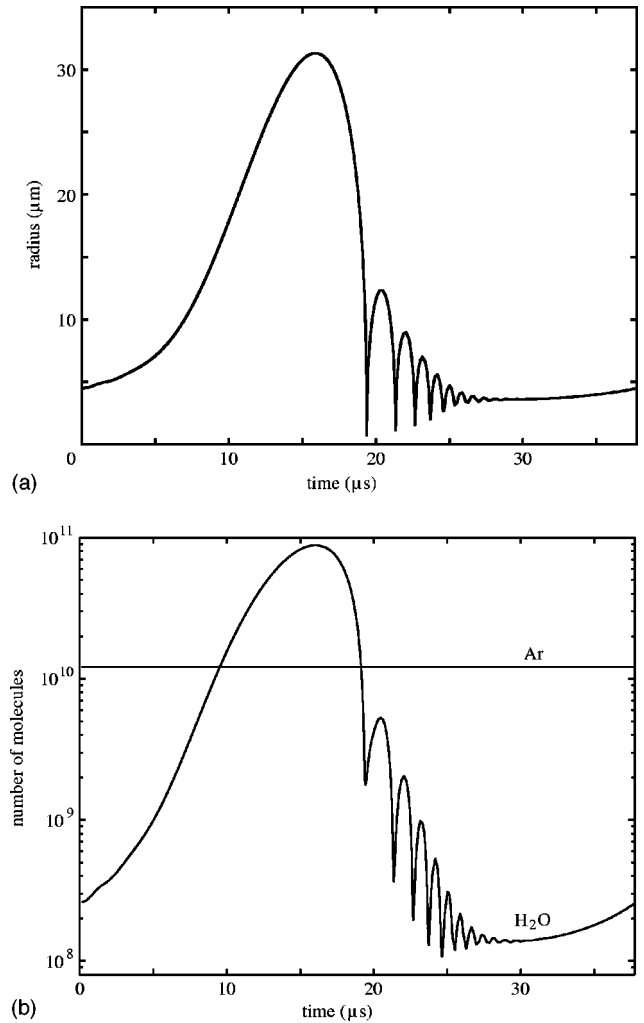
FIG. 24. Importance of water vapor exchange between bubble and fluid: (a) Bubble dynamics and (b) number of water molecules in the bubble as a function of time for an (initially) R_0=4.5\ \mu\text{m} argon bubble driven at P_a=1.2\ \text{atm} and f=26.5\ \text{kHz} . Note the comparison in (b) to the constant number of argon atoms. From Storey and Szeri (2000).
