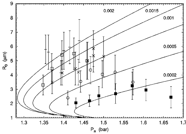
FIG. 34. Experimental data in the phase diagram in the P_a - R_0 plane: +, with an air concentration of c_{\infty}^{\text{air}}/c_0=0.2 ; \square , 0.15; \circ , 0.1; \blacksquare , 0.02. The data lie on the stable diffusive equilibria curves (solid lines) for argon concentrations of c_{\infty}^{\text{Ar}}/c_0=0.002 , 0.0015, 0.001, and 0.0002, confirming the argon rectification theory. Experimental data are taken for as large a P_a as possible, to probe the shape instability threshold. From Simon et al. (2001).
