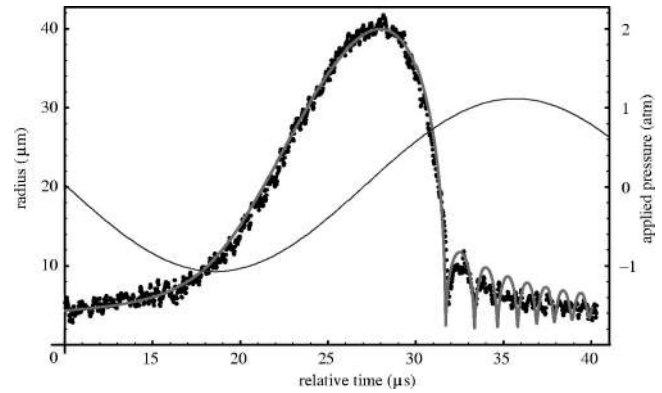
FIG. 21. Measured R(t) (with Mie scattering, dots) and a fit to these data based on the Keller equation (solid curve). The thin curve shows the driving pressure P(t) . From Matula (1999).
