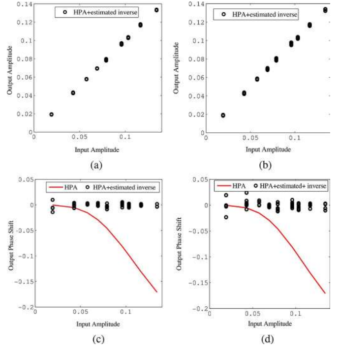
Fig. 4. Combined response of the true HPA and its estimated inversion obtained under OBO = 3 dB and E_b/N_o = 4 dB: (a) combined amplitude response by Scheme 1; (b) combined amplitude response by Scheme 2; (c) combined phase response by Scheme 1; and (d) combined phase response by Scheme 2.
