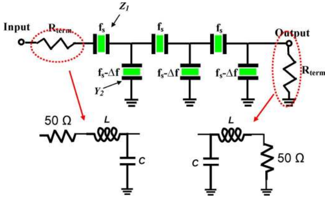
Fig. 3. Schematic representation of a ladder filter structure made out of three cascaded L networks. LC matching elements can be used to implement the termination resistance and directly couple the system match to 50 Ω.
