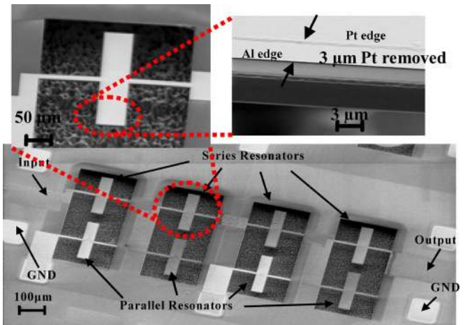
Fig. 13. SEM view of a ladder filter made out of eight electrically cascaded rectangular plate resonators. Zoomed-in view shows details of the single rectangular resonator and lithographically defined variation in bottom electrode length used to tune the center frequency of the series resonators.
