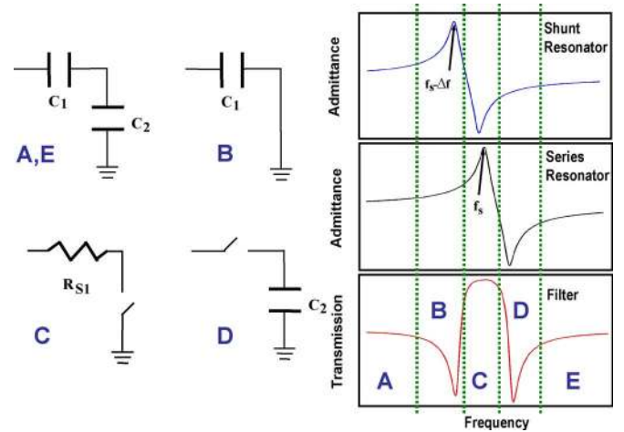
Fig. 5. Intuitive explanation of the principle of operation of the L section used as a building block in ladder filters. Five principle areas of operation have been identified and the corresponding equivalent circuit of each of the resonators has been highlighted.
