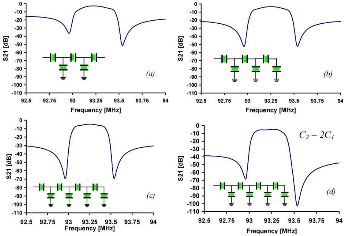
Fig. 6. Simulated S_{21} response of a 93-MHz filter implemented using rectangular plate resonators having individual Q of 2000 and R_M of 300 \Omega . The termination resistors were selected according to equation (5). (a) Electrical response of 3/2 ladder structure showing asymmetry and poor out-of-band rejection. (b) Electrical response of 3/3 ladder structure showing higher rejection and symmetrical response. (c) Electrical response of 4/4 ladder structure; higher out-of-band rejection is obtained, but insertion losses are increased with respect to (b). (d) Electrical response of 4/4 ladder structure for which a cap ratio of 2 between the parallel and series branches was selected [ C_1 and C_2 as defined in (3)]. This configuration improves out-of-band rejection with a small increase in insertion loss.
