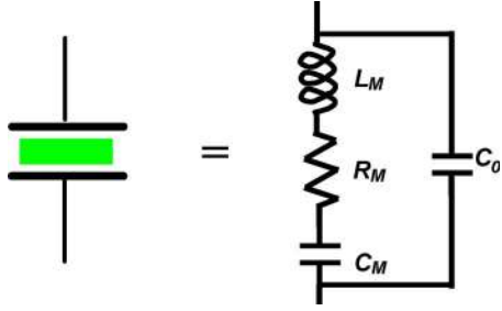
Fig. 2. Schematic representation of a piezoelectric resonator and equivalent BVD circuit representation.
