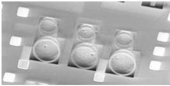
Fig. 12. Electrical response and SEM of a 236-MHz ladder filter realized using different size rings in the series and shunt branches.
