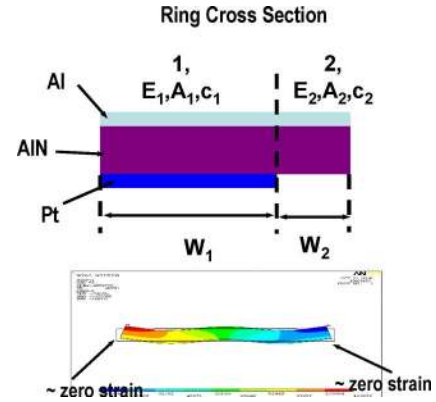
Fig. 7. Cross-sectional view of circular ring structure illustrating the location where Pt is lithographically removed in order to induce the desired frequency shift. Note that the Pt is removed at the location of minimum or almost zero strain as shown by cross-sectional view of resonator mode shape in ANSYS.
