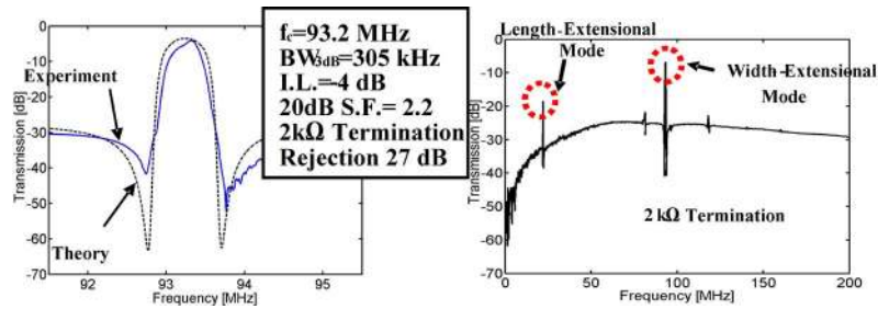
Fig. 14. Electrical response of a 93.2-MHz bandpass filter constituted by eight rectangular resonators arranged in a ladder configuration. Resonators had individual Q in the order of 2000. Large scan of the same filter response from 0 to 200 MHz with 2-k \Omega terminations was taken. A length-extensional mode is present together with the width-extensional mode.
