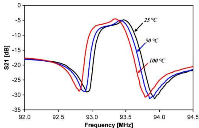
Fig. 16. Effect of temperature change (25–100 °C) on ladder filter composed of six rectangular plate resonators.
