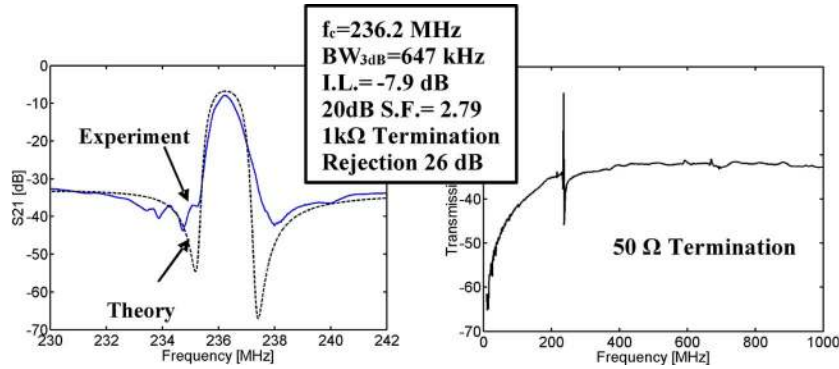
Fig. 11. Electrical response of a bandpass filter constituted by eight ring-shaped resonators arranged in a ladder configuration with termination of 1 k \Omega . The resonators had individual Q in on the order of 800. A large scan of the same filter showing no interfering spurious responses was taken from 0 to 1 GHz. 50- \Omega terminations were used in this scan (1-GHz-wide scan).
