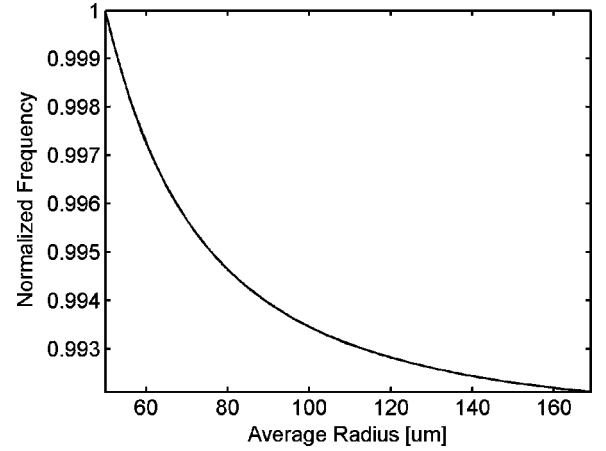
Fig. 8. Frequency variation versus average radius of a 20- \mu\text{m} -wide circular ring. Frequency is normalized to the value for a ring with 50- \mu\text{m} average radius. Rings with larger average radius have lower resonant frequency.
