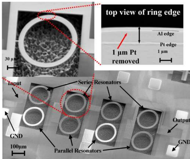
Fig. 10. SEM image of a fourth-order ladder filter made out of eight identical circular rings. The process-defined frequency shift defined by the removal of 1\text{ }\mu\text{m} of Pt from the series resonator is highlighted in the close-up views.
