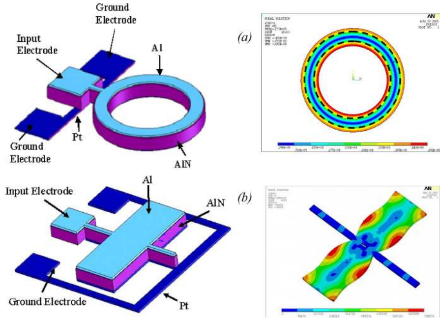
Fig. 1. Schematic views of the building blocks for the filters and their mode shapes. (a) Circular ring AIN resonator excited in a radial-extensional contour mode shape as shown in ANSYS plot. (b) Rectangular plate AIN resonator excited in a width-extensional contour mode shape as shown in ANSYS plot.
