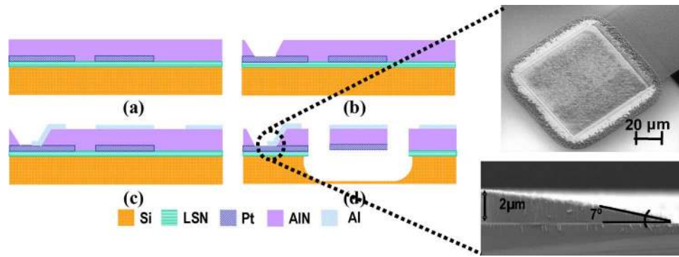
Fig. 9. Fabrication process used for the realization of ladder filters. (a) Low stress nitride (LSN) deposition by LPCVD, followed by Pt patterning by lift-off and AlN sputter deposition. (b) Open via access to bottom Pt electrode through AlN. AlN is wet etched by 160\text{ }^{\circ}\text{C} \text{H}_3\text{PO}_4 . (c) Deposition of top Al electrode and patterning by dry etching in \text{Cl}_2 -based chemistry. (d) \text{Cl}_2 -based dry etching of AlN resonant devices and dry release in \text{XeF}_2 . The inset SEMs show top and side views of the Al to Pt contact.
