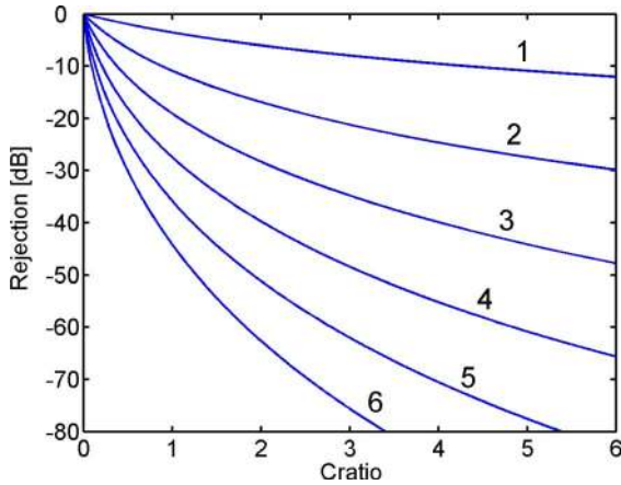
Fig. 4. Effect of capacitance ratio (between parallel and series branches) and number of L sections (here varying between 1 and 6) on the out-of-band rejection.
