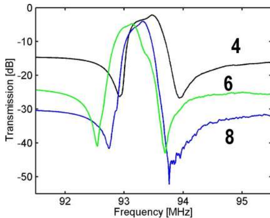
Fig. 15. Electrical response of second-, third-, and fourth-order ladder filters made out of, respectively 4, 6, and 8 rectangular plate resonators. Out-of-band rejection improves with filter order at the expenses of insertion losses.
