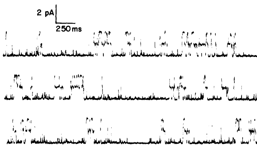
FIGURE 1. Dimeric bursts of \text{Cl}^- channels. A single \text{Cl}^- channel was inserted into a Montal-Mueller bilayer as described in Materials and Methods, and current was measured at -120 mV holding potential. In all traces in this report, upward deflection corresponds to channel opening.
