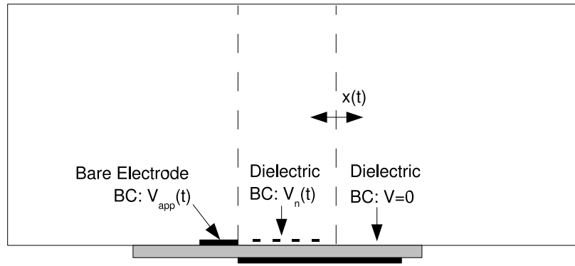
Figure 16: Computational domain for calculation of unsteady plasma body force.
