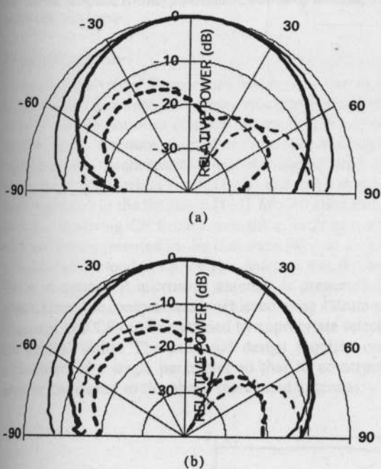
Figure 5 Measured E -plane and H -plane radiation patterns for the proposed antenna. (a) f_1 = 1411 MHz. (b) f_2 = 1611 GHz. — ..... E -plane, — ..... H -plane
