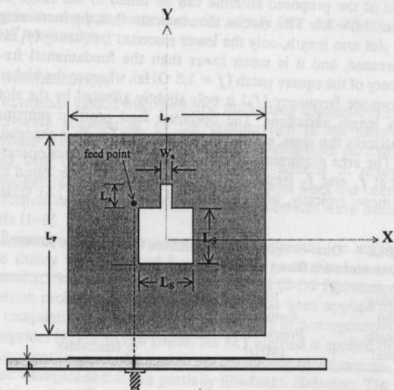
Figure 1 Geometry of the proposed dual-frequency dual-polarized slotted square microstrip antenna. Antenna parameters are given in Figure 2
