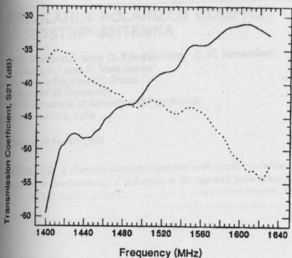
Figure 4 Variation of received power with frequency for the two orthogonal polarization planes. ----- vertical, — horizontal
