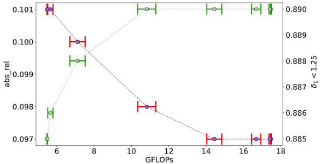
Figure 6: Analysis of performance vs decoder GFLOPs on KITTI. By adjusting the parameter \eta , we trade off computation in GFLOPs (x-axis) against accuracy (y-axis; Abs Rel in red, and \delta_1 in green). We show here that we can reduce the computation by more than half without any major degradation in accuracy.
