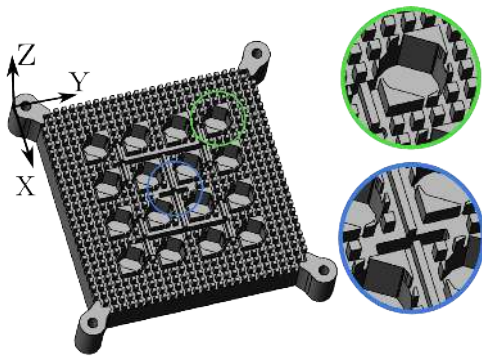
Fig. 12: 3D model of the 4 4 antenna. Detailed views of one cavity and the input are enlarged.
