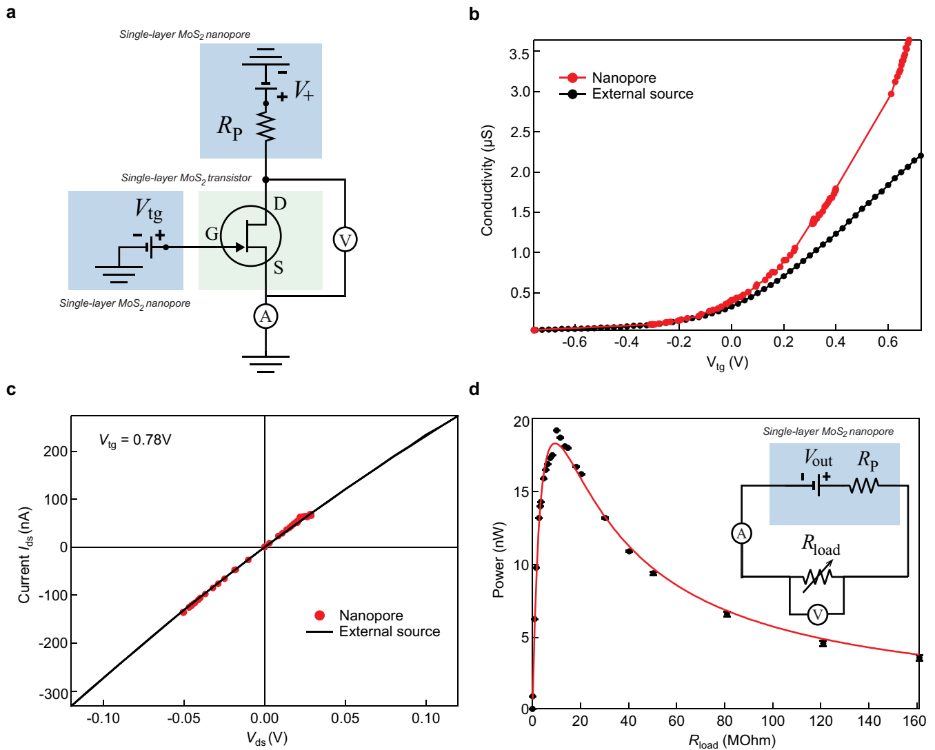
Extended Data Figure 8 | Characterization of a single-layer MoS 2 transistor with nanopores and SMU. a , Electrical measurements with two nanopores ( V_+ , nanopore output voltage; V_{ds} , drain–source voltage; V_{tg} , top gate voltage). The voltage drop across the transistor channel is monitored with the voltmeter (V); current is measured with current amplifier (A). b , Comparison of nanopore measurements with
