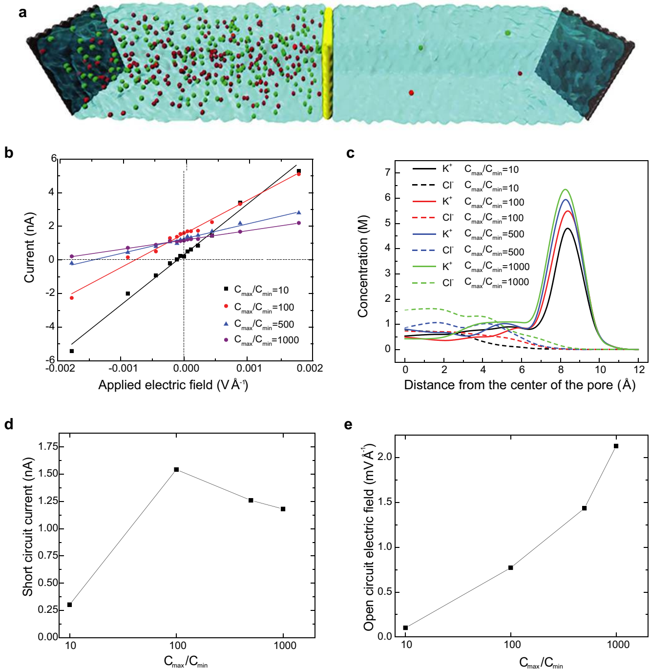
Extended Data Figure 4 | Molecular-dynamics simulations of power generation for various ratios of concentration gradients. a , A typical simulation box. b , Current as a function of the applied electric field for a single-layer \text{MoS}_2 , at different concentration ratios. c , \text{K}^+ and \text{Cl}^-
