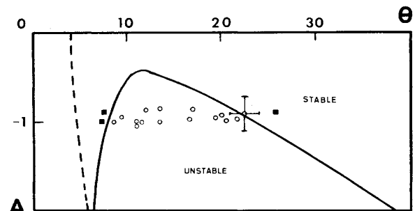
FIG. 17. Domain of instability in the detuning space for C=60\pm 5 , \kappa'=0.5 , and \gamma=1.6 . Open circles indicate instability, closed squares stability. Below the continuous line is the unstable region based on the Gaussian theory, while to the right of the dashed line is the plane-wave prediction of the unstable region. The ring cavity c is used in this measurement. Systematic uncertainties in the detunings are \pm 10\% .
