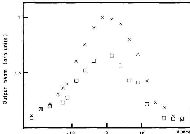
FIG. 15. Transverse profile of the output beam. The \times 's represent the average power as a function of aperture position when the system is self-pulsing ( C=50\pm 10 , \Theta=-21\pm 1 , \Delta=-2\pm 0.5 , \kappa'=0.32 , and \gamma=1.6 ). The squares are the output of the rf mixer as a function of aperture position; this signal is proportional to just the oscillatory part of the output beam and to any phase difference between the spatially resolved oscillations and the whole beam oscillations. Measurements done with cavity e .
