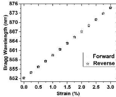
Fig. 5. Strain response of single-mode SIPOFBG.
