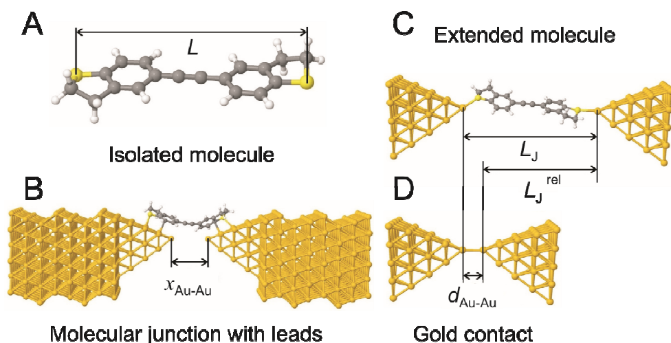
Figure 6. Schematic representation of the “extended molecule” of BTI in contact with conducting leads. The Figure illustrates the relevant distances and lengths L , x_{\text{Au-Au}} , L_J , d_{\text{Au-Au}} and L_J^{\text{rel}} , which were computed after the DFT-based structure has relaxed. L is the distance from the centre of an anchor atom at one end of the fully-extended isolated molecule to the centre of the anchor atom at the other end. At an arbitrary stage during the theoretical junction stretching, the theoretical electrode separation x_{\text{Au-Au}} is defined as the distance between the center of the two gold apex atoms. L_J is defined to be the value of x_{\text{Au-Au}} when the junction breaks. The distance d_{\text{Au-Au}} 0.25 nm is the electrode separation of a monatomic gold contact, when the junction has the conductance G_0 . This is the gold-gold distance at which the bond between apex atoms is neither compressed nor stretched. L_J^{\text{rel}} is the theoretically estimated relative displacement of a junction containing a fully extended molecule, arising when the zero of relative displacement ( \Delta z = 0 ) corresponds to an apex-atom separation of d_{\text{Au-Au}} and is defined as L_J^{\text{rel}} = L_J - d_{\text{Au-Au}} (see SI Table S2). Panel B shows the structure of the gold electrodes used in the simulations.
