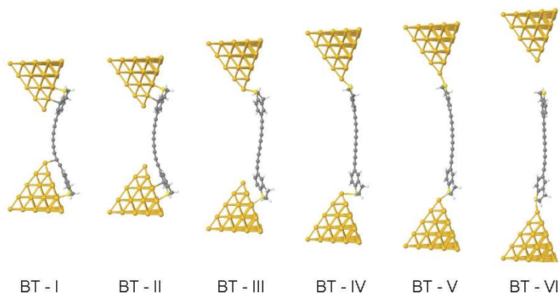
Figure 7. Examples of junction evolution of oligoynes derivatives BT4 showing key configurations.
