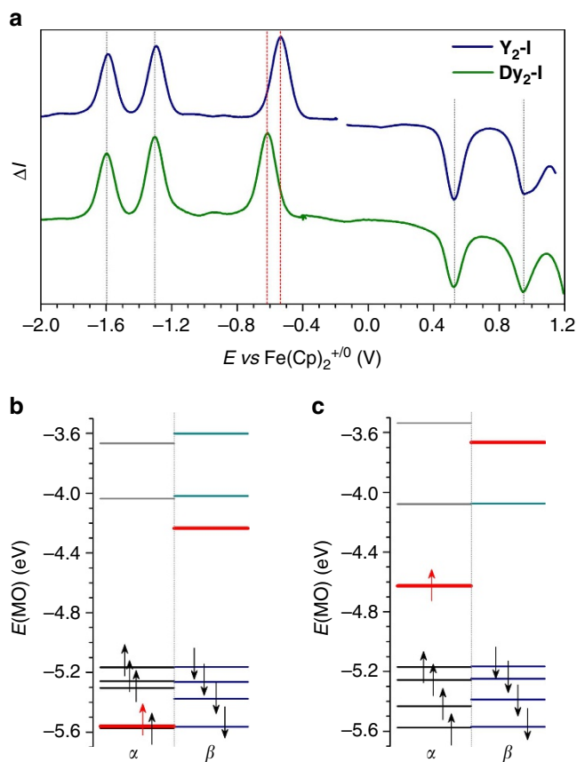
Figure 4 | Electrochemical properties and frontier MOs. (a) Square wave voltammetry of \text{Y}_2\text{-I} and \text{Dy}_2\text{-I} in 0.1 M \text{TBABF}_4/\text{o-dichlorobenzene} , vertical bars show positions of redox potentials (black for identical potentials in the two EMFs, red for the metal-based first reduction potentials found at -0.52 \text{ V} in \text{Y}_2\text{-I} and -0.60 \text{ V} in \text{Dy}_2\text{-I} ). (b) DFT-computed MO levels in \text{Y}_2\text{-I} , spin-up ( \alpha ) and spin-down ( \beta ) levels are shown separately; arrows denote electrons in occupied MOs; two components of the M-M bonding single-occupied MO are shown in red. (c) The same as (b) but for \text{La}_2\text{-I} . It is noteworthy that the energies of the M-M bonding MOs in \text{La}_2\text{-I} are considerably higher than those in \text{Y}_2\text{-I} .
