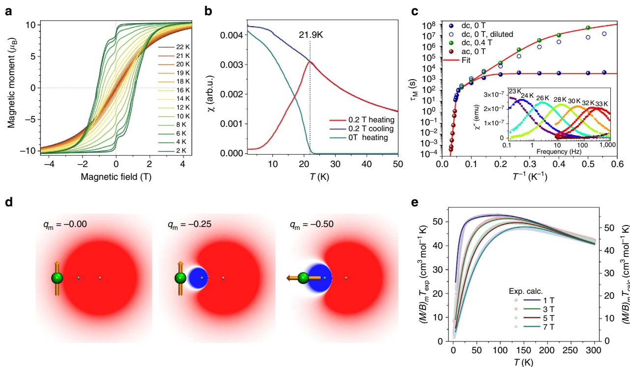
Figure 5 | Magnetic properties of Dy 2 -I. (a) Magnetization curves measured at various temperatures with the field sweep rate of 2.9 mT s -1 . (b) Determination of blocking temperature T_B : the sample is first cooled in zero-field to 1.8 K, then \chi is measured in the field of 0.2 T with increasing temperature at the heating rate of 5 K min -1 (red curve), then the measurement is performed at cooling down to 1.8 K (blue curve); finally, the field is turned off and decay of \chi is measured at increasing temperatures (cyan curve). The vertical bar denotes T_B . (c) Magnetization relaxation times obtained from dc- and ac-measurements (dots), solid curve is a global fit using equations (1-2). The inset shows \chi'' values measured at different temperatures and frequencies (dots), solid lines are result of the fitting with a generalized Debye model. (d) Evolution of crystal field potential and the type of Dy 3+ anisotropy in the system comprising 3 + point charge placed at the distance of 3.96 Å and an additional negative charge ( q_m ) placed at the midpoint between the two Dy centres. Dy is shown as a green sphere, the arrow denotes direction of the magnetic moment. (e) Experimental and computed (M/B)_m T curves (dots and lines, respectively) for the fields of 1, 3, 5 and 7 T. Computations were performed using the effective spin Hamiltonian in equation (4) with j_{Dy,e} = 32 \text{ cm}^{-1} (46 K). Experimental values are systematically smaller than theoretical one by a factor of 1.05; hence, the scales are slightly different.
