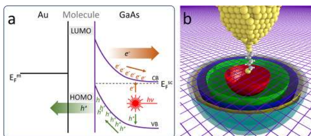
Figure 3. (a) Schematic band diagram for the illuminated MMS junction under reverse bias and (b) simplified depiction of the hemispherical space charge region at different bias values. The ideal space charge region is a red hemisphere at low bias, incrementing through green, blue, and yellow to cyan at higher bias. GaAs surface is represented as a purple mesh for clarity.
