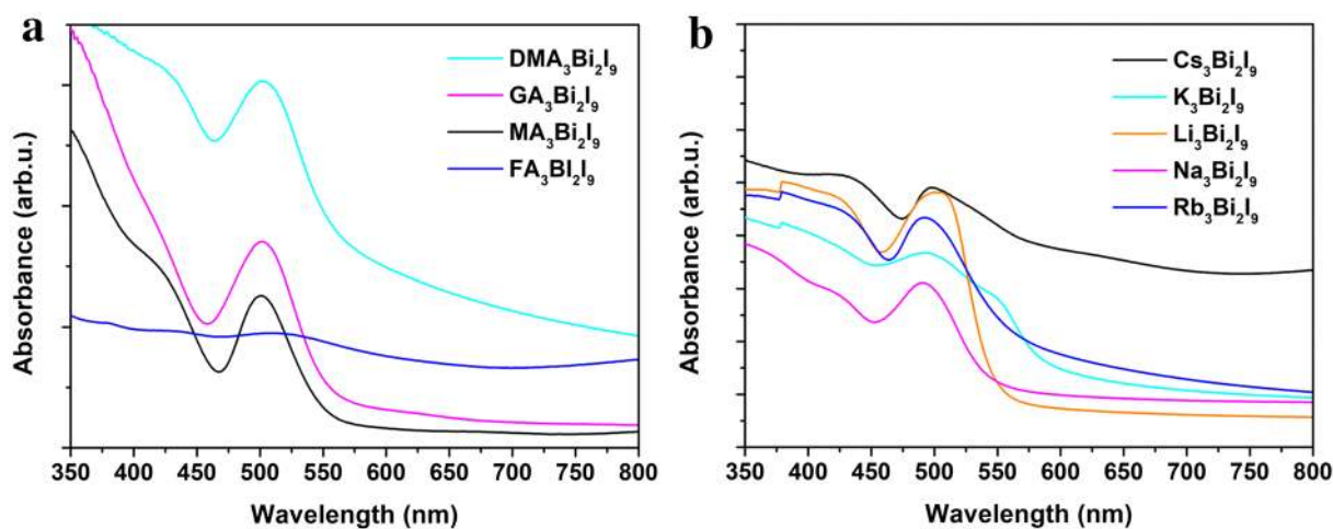
Figure 3: UV-Vis absorption spectra of A 3 Bi 2 I 9 thin films with (a) organic A-site cations and (b) inorganic A-site cations.
