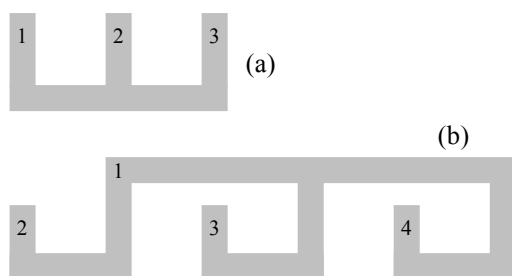
Figure 3: Chaining effect of multiple merges: (a) 1 \Rightarrow 2 ; 2 \Rightarrow 3 ; subsequent label 1s require multiple merger table lookups. (b) Merging left counter-example: 1 \Rightarrow 2 ; 1(2) \Rightarrow 3 ; 1(2) \Rightarrow 4 resulting in an incorrect merger table.
