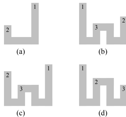
Figure 4: Merging scenarios: (a) the smaller label on right; (b) – (d) the smaller label on the left in the first merger.
