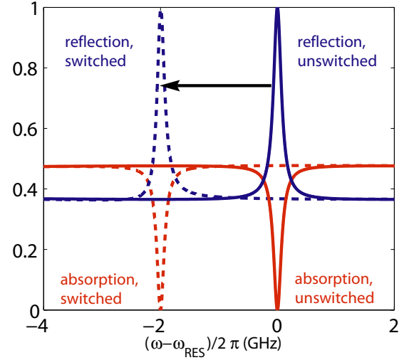
FIG. 3. (Color) Waveguide reflection (blue) and absorption (red) in the absence (solid) and presence (dashed) of a control photon, demonstrating nonlinear single-photon switching ( \Gamma_w=21.5 GHz, g_{13}=20.5 GHz, \Omega_c=2 GHz, \Gamma_3=30 GHz, g_{24}=8 GHz, and \Delta\tilde{\omega}_{24}=30 GHz).
