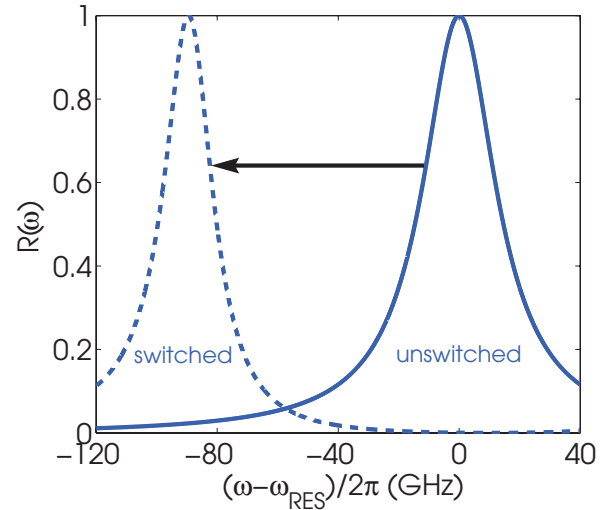
FIG. 5. (Color) Waveguide reflection with (dashed) and without (solid) a control photon, demonstrating lossless switching, where multiple (49) EIT atoms have been used to push the Rabi-split peaks farther away in the presence of negligible loss ( \Gamma_w=21.5 GHz, g_{13}=143.5 GHz, \Omega_c=210 GHz, \Gamma_3=0 GHz, g_{24}=210 GHz and \Delta\tilde{\omega}_{24}=20 GHz).
