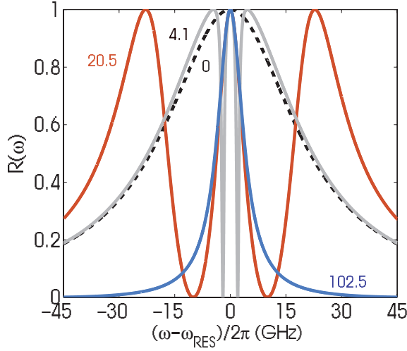
FIG. 2. (Color) Waveguide reflection for a lossless three-level EIT atom for the four labeled values of the atomic coupling strength g_{13} (in gigahertz). The radiation rate \Gamma_w=21.5 GHz and the ratio g_{13}/\Omega_c=2 are fixed. Larger g_{13} produces larger peak separations (the blue curve shows Rabi peaks outside of the plot), favorable for switching.
