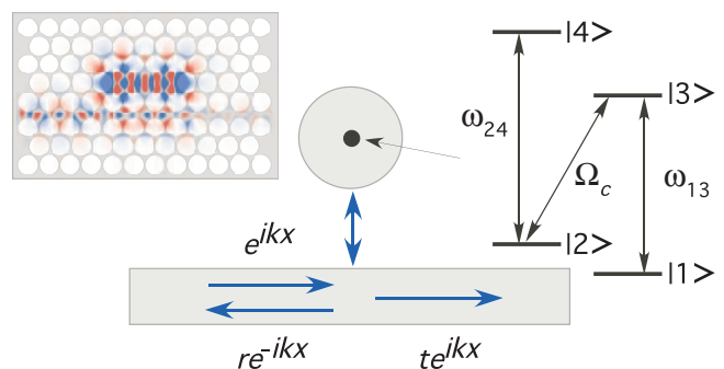
FIG. 1. (Color) Schematic illustration of the system investigated. A waveguide is coupled to a cavity with an EIT atom at its center. In the upper left-hand corner, an FDTD simulation that can be used to calculate the model parameters is shown.
