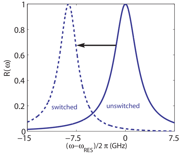
FIG. 4. (Color) Waveguide reflection with (dashed) and without (solid) a control photon, demonstrating lossless switching, where a higher quality factor has made the resonant peaks narrow enough to be shifted by more than their full width at half maximum by a single photon ( \Gamma_w=3 GHz, g_{13}=20.5 GHz, \Omega_c=30 GHz, \Gamma_3=0 GHz, g_{24}=30 GHz, and \Delta\tilde{\omega}_{24}=20 GHz).
