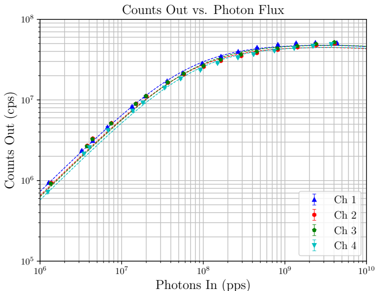
Figure 3: Output count rate vs. input photon flux.
