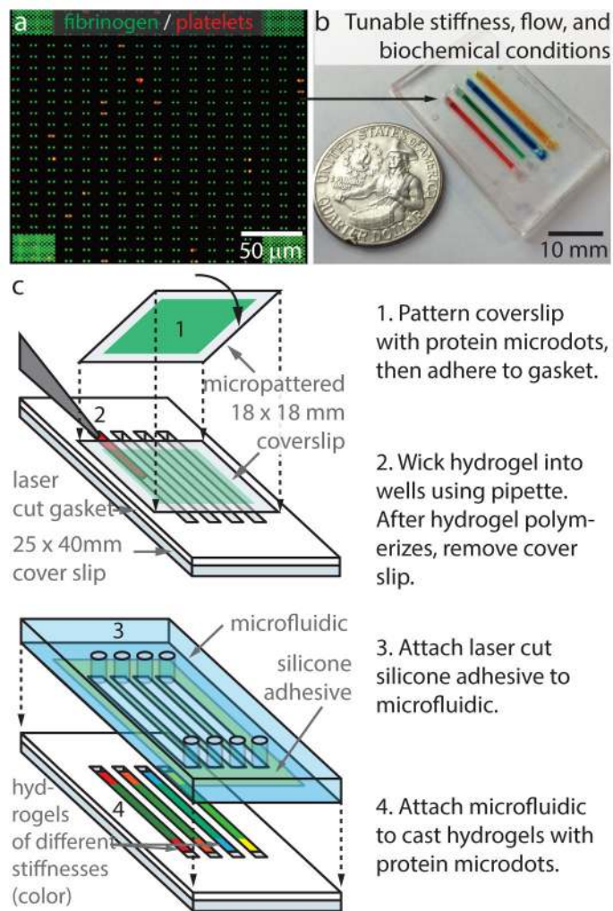
Figure 2. Platelet contraction cytometer - hydrogels with microprinted arrays of fibrinogen microdots are encapsulated in separate microchannels, enabling the biochemical, mechanical, and shear microenvironments to be precisely controlled and varied simultaneously. a , A confocal image showing single platelets (red, contracting against fibrinogen microdot pairs (green) on the hydrogel surface. Over 20,000 fibrinogen microdot pairs are microprinted on the surface of each hydrogel encapsulated in each microchannel. b , Each microfluidic device may comprise different variables, here four of microchannels comprise of hydrogels of different stiffness. c , A novel yet relatively simple fabrication process flow enables rapid manufacturing.
