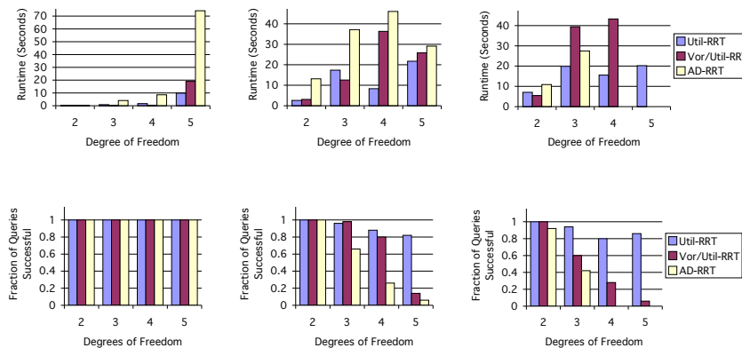
Fig. 4. Average run times (top row) and success rates (bottom row) for different algorithms on large, medium, and small bug traps (relative to the configuration space size)
