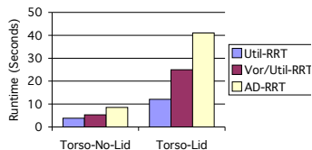
Fig. 6. Average run time of various planning algorithms for the 14-DOF humanoid torso in two different environments
