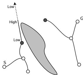
Fig. 2. An illustration of utility for expansion distance. Expansion beyond the shadow of the obstacle does not increase the utility of the expansion.
