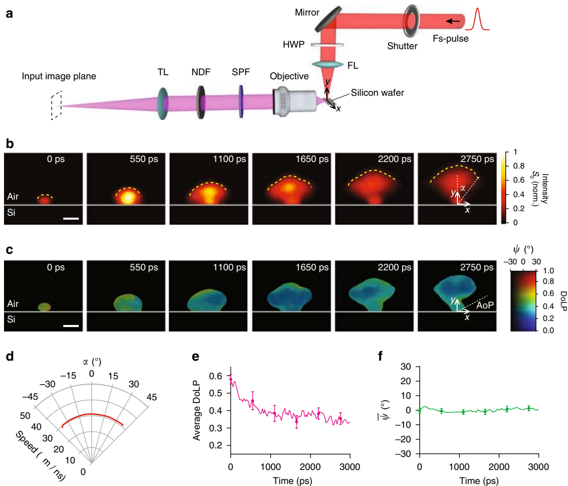
Fig. 3 Spatiotemporally resolved polarization imaging of the plasma dynamics from the laser-induced breakdown on a silicon wafer. a Experimental setup. The incident pulse was polarized in the x direction. FL, focusing lens; HWP, half-wave plate; NDF, neutral density filter; SPF, short-pass filter; TL, tube lens. Equipment details are in Methods. b Normalized intensity ( S_0 ) dynamics of a plasma plume. The gray line in each panel represents the air-silicon interface. The yellow dashed line represents the plasma plume front. The full sequence is shown in Supplementary Movie 2. c Spatiotemporally resolved DoLP and AoLP ( \psi ). In the 2D colormap, the jet and grayscale colormaps are used for DoLP and AoLP, respectively. d Plasma plume expansion speed over angle \alpha , which is defined in b . e Spatially averaged DoLP over time. f Spatially averaged \psi over time. Scale bars in b and c : 50 \mu\text{m} . Error bars in e and f represent standard deviations of DoLP and \psi in the spatial domain at the six snapshots shown in c .
