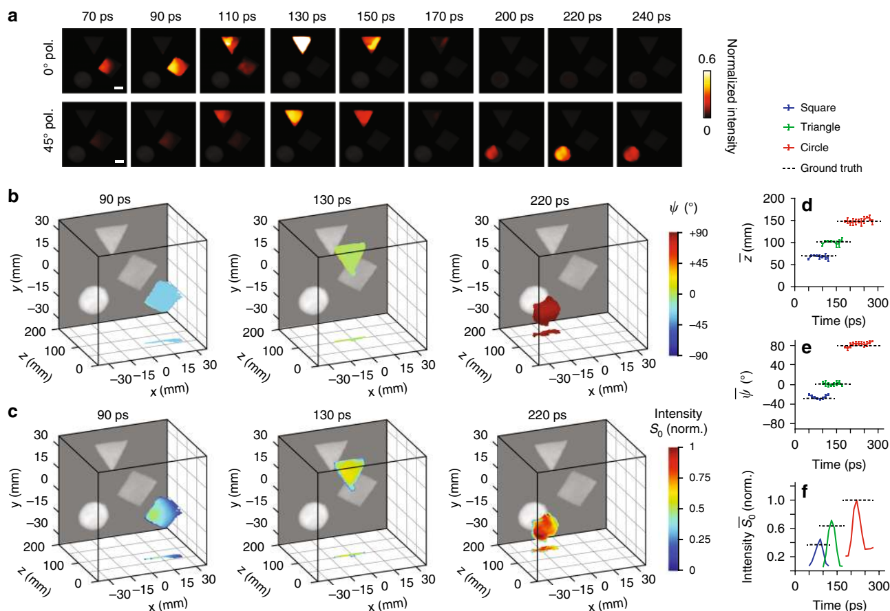
Fig. 4 Stereo-polarimetric ultrafast ( x, y, z, t, \psi ) imaging using SP-CUP. a Nine representative frames of the ultrafast dynamics imaged at 100 Gfps using Views 1, 3, and 4 (top row) through the 0^\circ polarizers and Views 2, 5, and 6 (bottom row) through the 45^\circ polarizers. The full evolution is in Supplementary Movie 4. b–c Reconstructed AoLP ( \psi ) b and the first Stokes parameter ( S_0 ) c in 3D space at three representative frames: 90 ps, 130 ps, and 220 ps. A relative depth is used by setting the 600-mm depth as the origin. The back side of the plot is the time-unsheared image. The images on the x - z plane are the projections of the 3D plots along the y axis. d–f Averaged values of z d , \psi e and S_0 f of the three shapes versus time. The black dashed lines are the ground truths measured using the time-unsheared stereo images from the external CCD cameras (Views 1 and 2). Note that the finite lengths of these dashed lines are for illustration only and do not indicate durations of events. Scale bar in a , 10 mm. Error bars in d and e , standard deviations.
