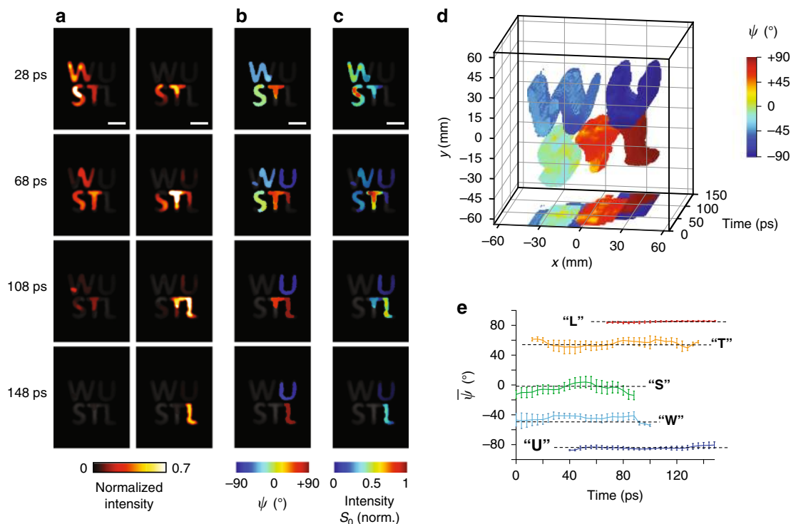
Fig. 2 Plano-polarimetric ultrafast ( x, y, z, t, \psi ) imaging using SP-CUP. a Representative frames of the reconstructed ultrafast dynamics at 250 Gfps from Views 1, 3, and 4 with the 0^\circ polarizers (left column) and Views 2, 5, and 6 with the 45^\circ polarizers (right column). The full sequence is in Supplementary Movie 1. These frames are overlaid on top of the time-unsheared image (grayscale) captured by the external CCD camera (Views 1 and 2). Note that the colormap is saturated at 0.7 in order to better display weak intensities. b, c Representative frames of the reconstructed AoLP ( \psi ) b and the first Stokes parameter ( S_0 ) c . d Evolutions of \psi in the x - y plane. The projection on the x - t plane is plotted at the bottom. e Averaged values of \psi for the five letters over time. The black dashed lines are the ground truths measured using the time-unsheared images (Views 1 and 2). Note that the finite lengths of these dashed lines are for illustration only and do not indicate durations of events. Error bars in e , standard deviations. Scale bars in a-c , 30 mm.
