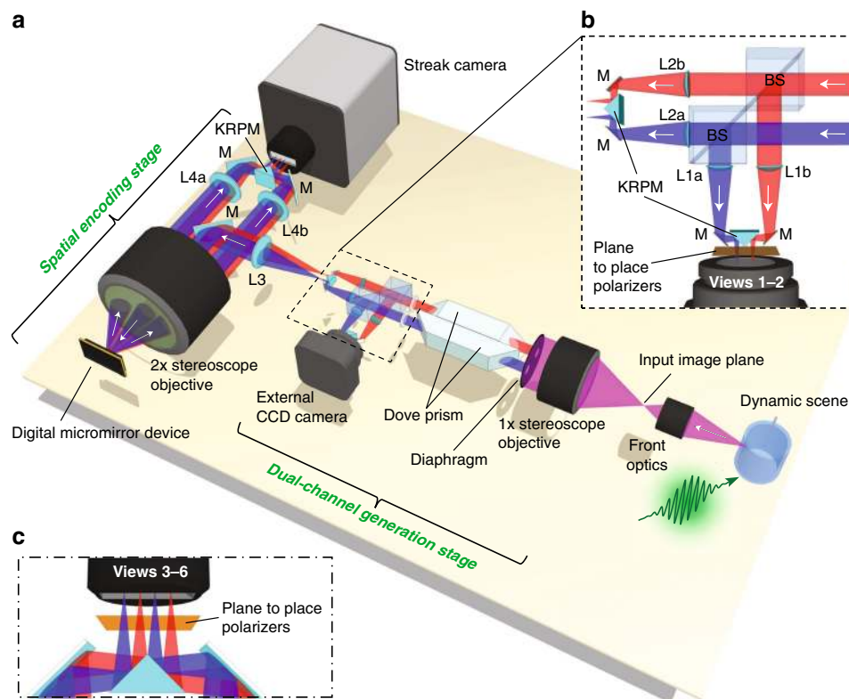
Fig. 1 Schematic of the SP-CUP system. BS, beamsplitter; L1a–L4b, Lenses; M, mirror; KRPM, knife-edge right-angle prism mirror. a The entire SP-CUP system. b Detailed illustration of beam splitting and polarization filtering in dual-channel-generation stage (dashed box). c Detailed illustration near the streak camera's entrance port. Equipment details are listed in Methods.
