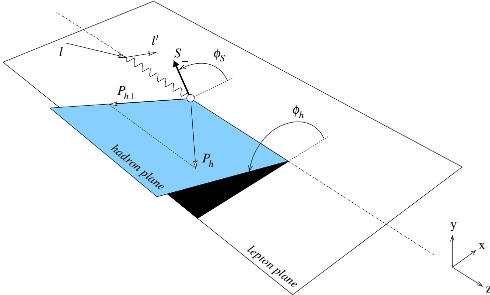
FIG. 1: Definition of azimuthal angles for the process (15) in the target rest frame. P_{h\perp} and S_{\perp} are the components of P_h and S transverse to the photon momentum.
