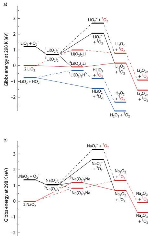
Fig. 5 Reaction free energy profiles for superoxide disproportionation. (a) LiO_2 disproportionation with itself, O_2^- or HO_2 to Li_2O_2 and molecular oxygen. (b) NaO_2 disproportionation with itself or O_2^- to Na_2O_2 and molecular oxygen. Pathways to release ^3O_2 and ^1O_2 are indicated by full and dashed lines, respectively. All species are computed in the solvated state except for the final solid peroxide. The computational method is M06-2X6-31**G++C-PCM ( \epsilon = 7.28 ). Numerical values are given in Tables S2–S4 (ESI † ). Further asymmetric alkali superoxide pairings are considered in Supplementary Note 5 (ESI † ).
