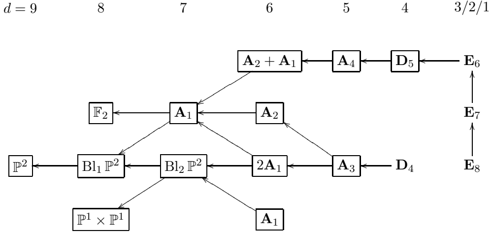
FIGURE 1. Generalised del Pezzo surfaces S defined over \bar{k} that satisfy \#\{\text{negative curves on } S\} \leq \text{rk Pic}(S) . The boxed ones are equivariant compactifications of \mathbb{G}_a^2 . Arrows denote blow-up maps.
