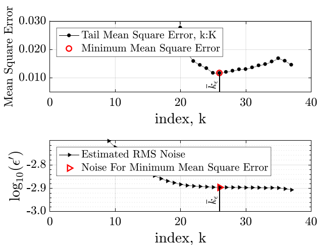
(b) Tail Matching Metrics
