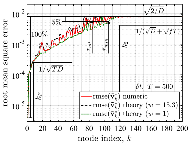
(b) RMSE ( \delta t, T = 500 case)
