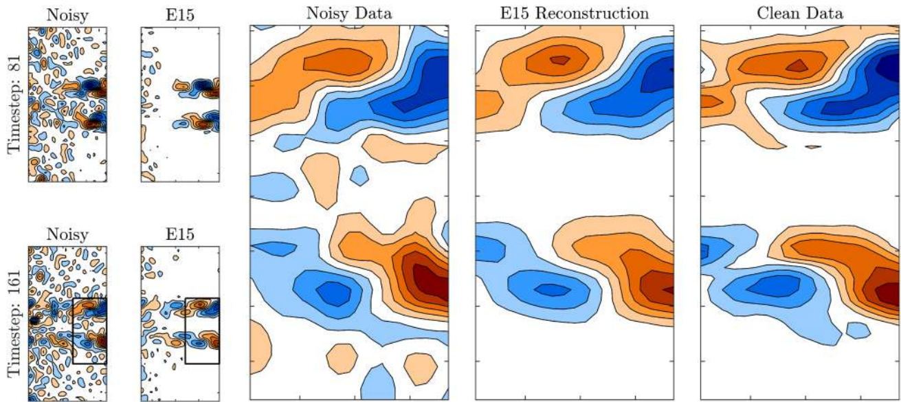
Fig. 12 (Sect. 6 Laminar Jet PIV example) Snapshots of vorticity (with time-mean flow removed). The small panels show the noisy data and ‘ \bar{\mathbf{u}}_{\rho} \bar{s}_{\rho} \bar{\mathbf{v}}_{\rho} ’ E15’ reconstruction ( \bar{r}_{\min} = 30 ) at two times ( t = 81
