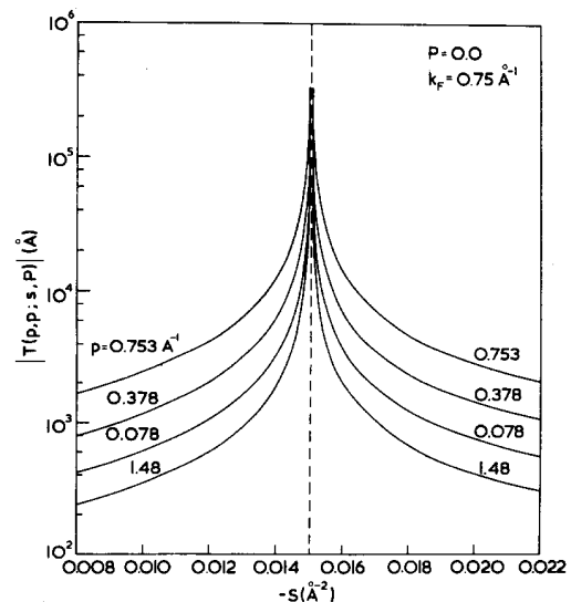
FIG. 1. S -wave GF T matrix for the MFM potential as a function of s , for four values of the diagonal relative momentum.
