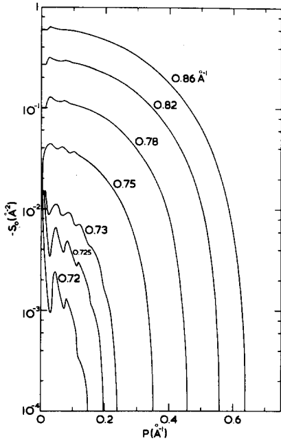
FIG. 2. Position of the singularity s_0 in the S-wave GF T matrix for the MFM potential as a function of the c.m. momentum P , for seven values of k_F .
