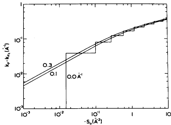
FIG. 3. Fermi momentum k_F vs the position of the singularity s_0 in the S-wave GF T matrix for the MFM potential, for three values of the c.m. momentum P=0.0, 0.1, \text{ and } 0.3 \text{ \AA}^{-1} , for which the critical values k_{F_c} are, respectively, 0.7146, 0.7158, \text{ and } 0.7375 \text{ \AA}^{-1} .
