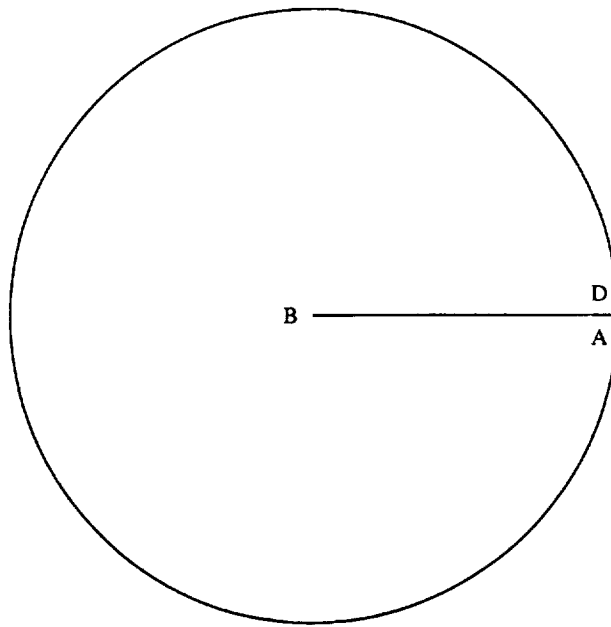
1. Fig. 1: The complex \zeta cut unit circle.
