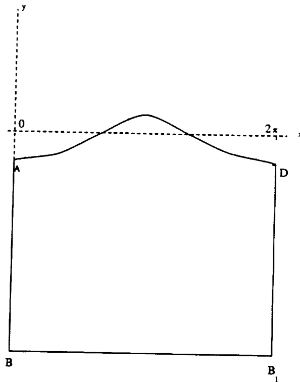
4. Fig. 4: The physical z = x + iy plane for finite depth water waves.
