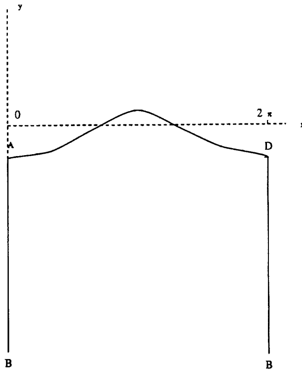
2. Fig. 2: The physical z = x + iy plane.
