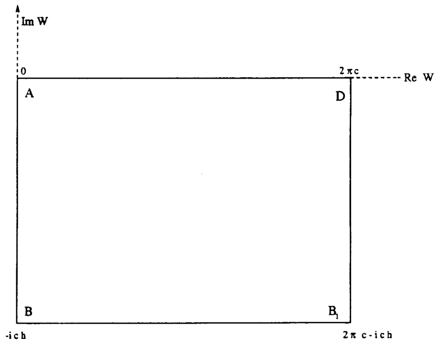
6. Fig. 6: W plane corresponding to finite depth steady water waves.
