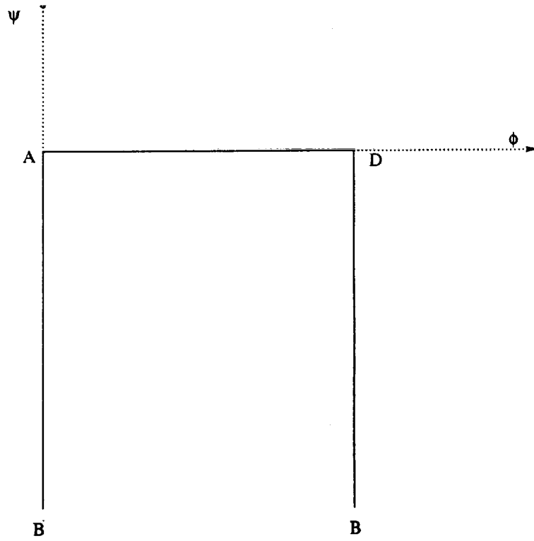
5. Fig. 5: W = \phi + i\psi plane for steady deep water wave.
