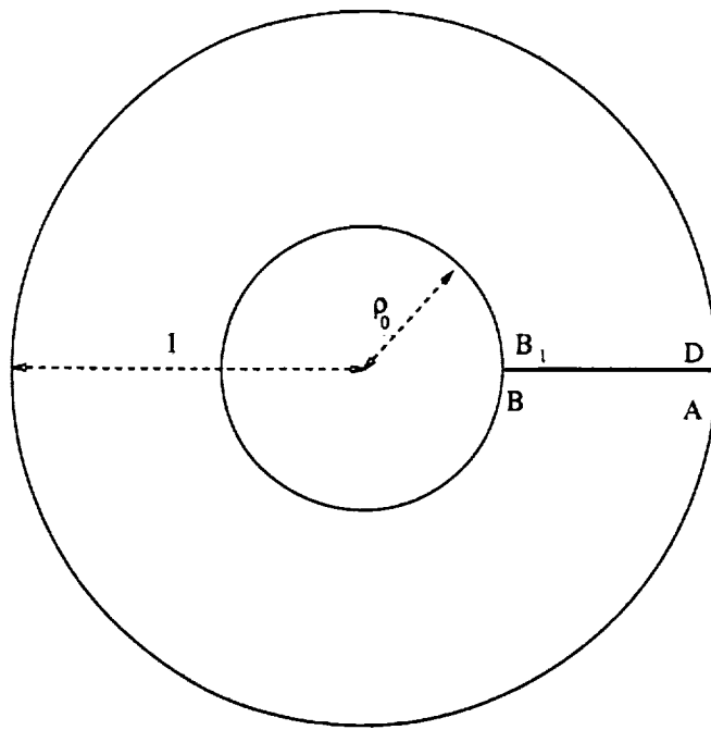
3. Fig. 3: The \zeta annular region with a cut corresponding to finite depth water waves.
