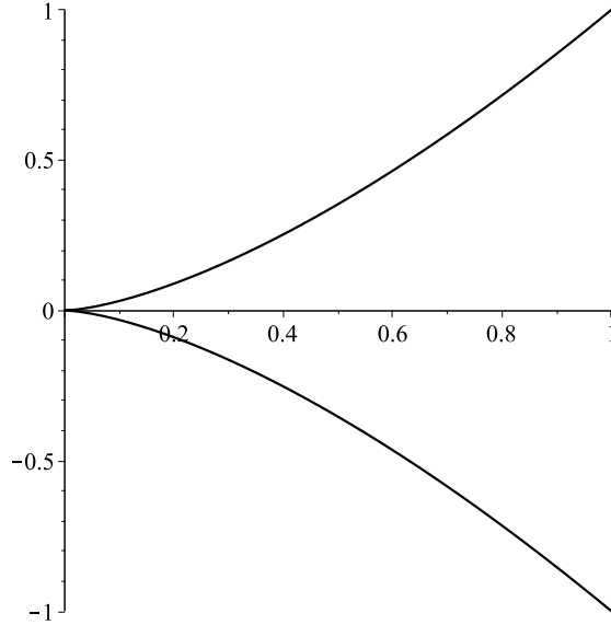
FIG. 4. The cusp (t^2, t^3)
