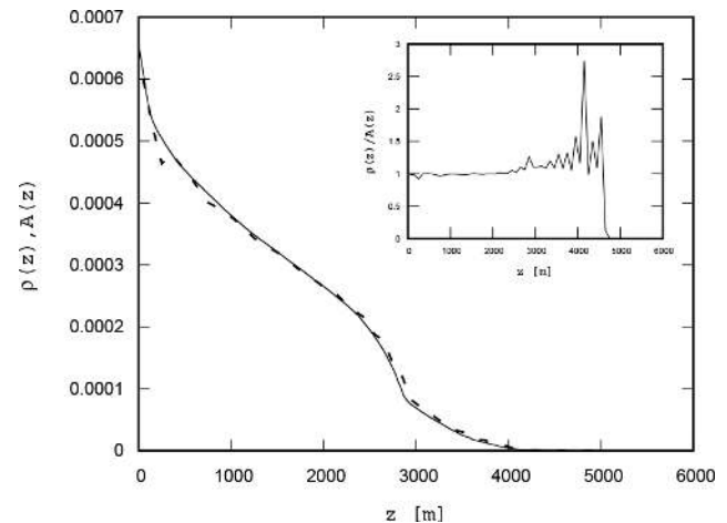
Figure 5. The continuous line is the area that the Mediterranean has at each depth z . The dashed line is microplastic density per unit of depth \rho(z) under continuous release of particles with \beta = 0.8 at 1 m depth. Both curves have been normalized to have unit area, so that they can be compared on the same scale. The binning size is 100 m. The inset shows the ratio \rho(z)/A(z) , proportional to the mass density of microplastic per unit of volume \rho_V(z) .
