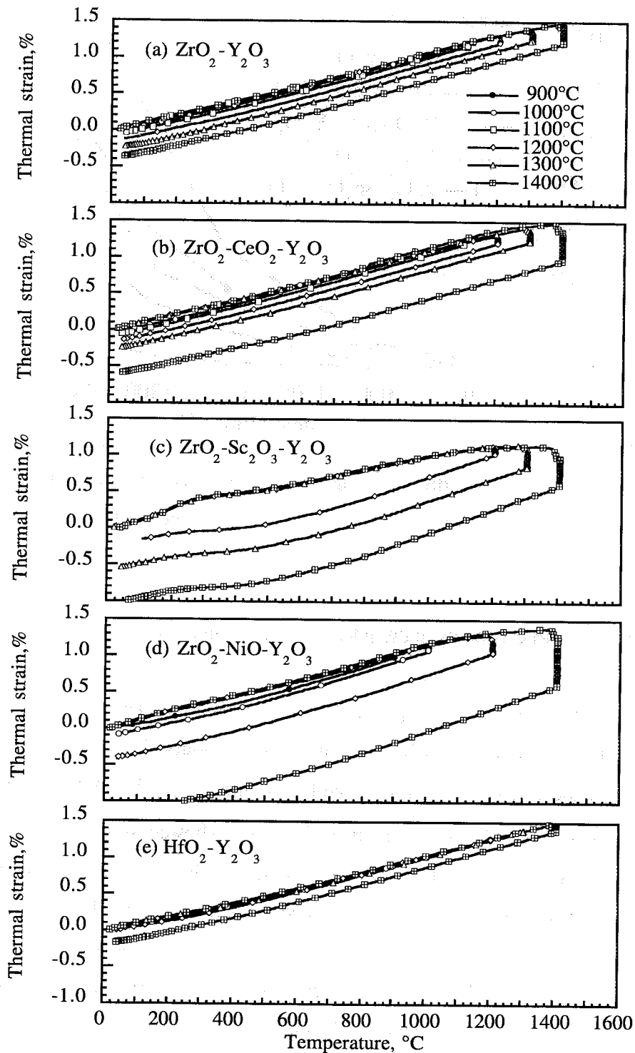
Fig. 2 Thermal expansion and sintering shrinkage response for the coating materials during the dilatometry sintering experiments at various temperatures. (a) ZrO_2 -8wt% Y_2O_3 ; (b) ZrO_2 -25wt% CeO_2 -2.5wt% Y_2O_3 ; (c) ZrO_2 -6wt% Sc_2O_3 -2wt% Y_2O_3 ; (d) ZrO_2 -6wt% NiO -9wt% Y_2O_3 ; (e) HfO_2 -27wt% Y_2O_3 .
