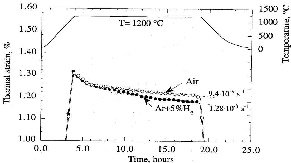
Fig. 5 Sintering shrinkage kinetics of plasma-sprayed \text{ZrO}_2\text{-}8\text{wt}\%\text{Y}_2\text{O}_3 at 1200^\circ\text{C} in air and in \text{Ar}+5\%\text{H}_2 .
