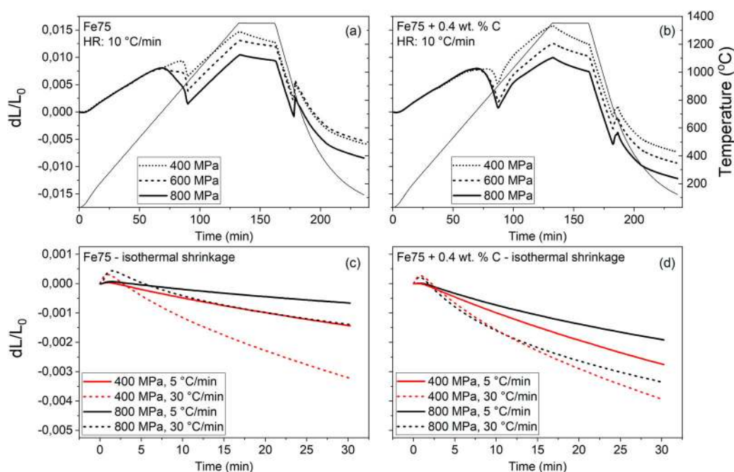
Figure 4. Fe75 sintering cycle matrix. (a) Varying compaction pressure at 10^\circ\text{C min}^{-1} , (b) with added carbon. (c) Isothermal shrinkage at 1350^\circ\text{C} for four sintering conditions, (d) with added carbon.
