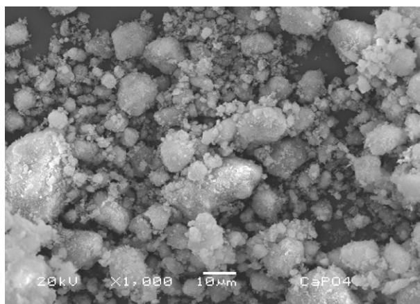
Fig. 4. Micrograph and elemental microanalysis X-ray spectrum of calcium phosphate
