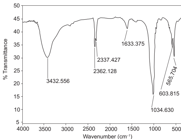
Fig. 1. IR spectrum of calcium phosphate
