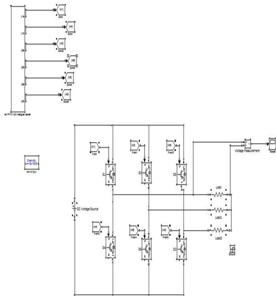
Fig:1 Circuit for sinusoidal pwm
