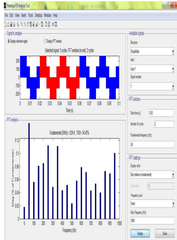
Fig:6 fft analysis of svpwm
