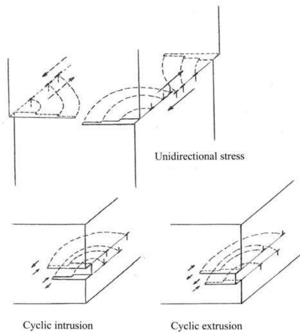
Fig. 6. Cyclically-induced slip intrusions/extrusions and internal dislocation structures.
