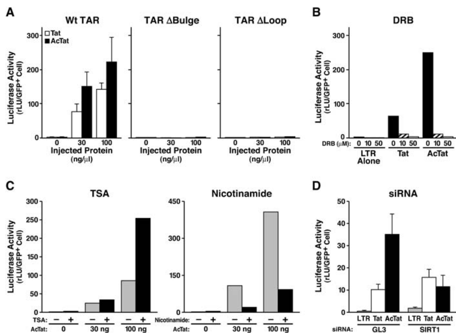
Figure 5. Transcriptional Activity of AcTat Depends on Deacetylation by SIRT1
