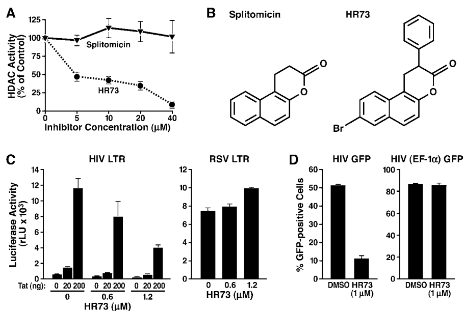
Figure 6. Inhibition of HIV Gene Expression by a Small Molecule Inhibitor of SIRT1
