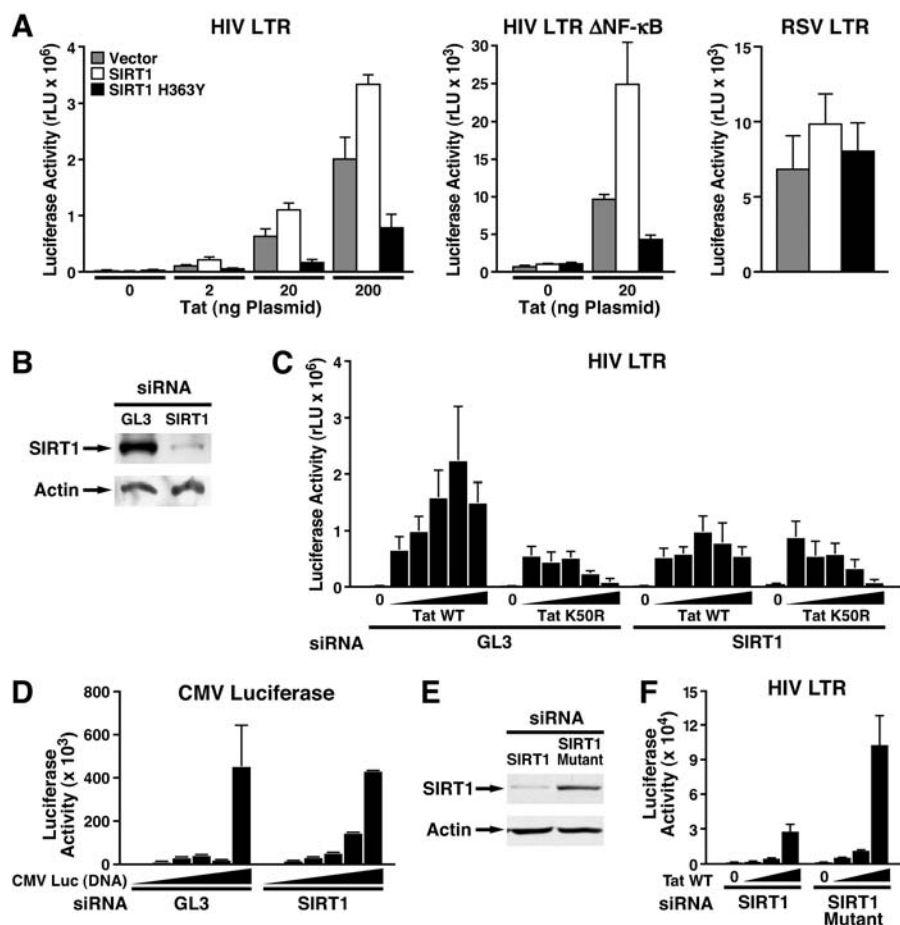
Figure 3. SIRT1 Is a Positive Cofactor for Tat Transactivation
