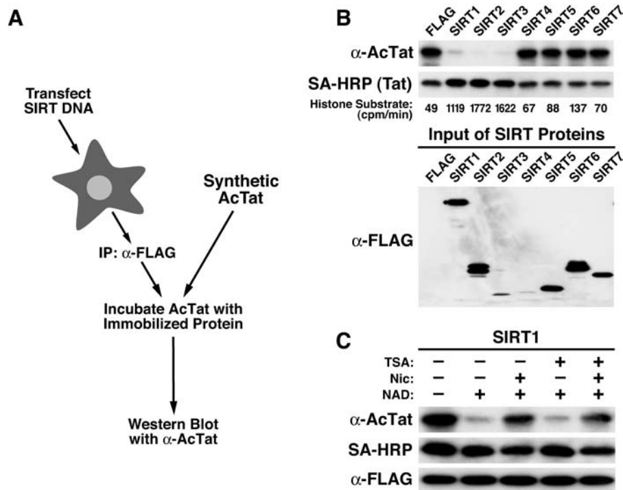
Figure 1. In Vitro Tat Deacetylation by Human SIRT Proteins
