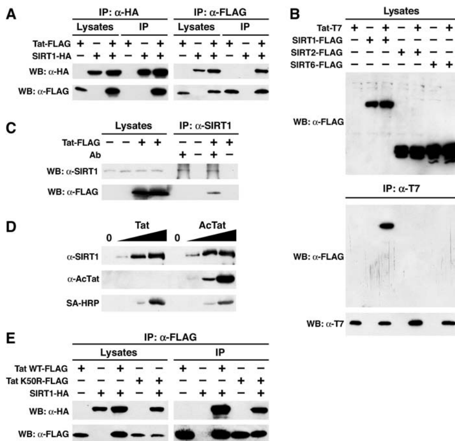
Figure 2. Physical Interaction between Tat and SIRT1
