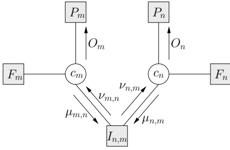
Fig. 2. Detail of the factor graph corresponding to (12) and relevant notation for the propagated messages.
