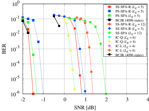
Fig. 6. Performance over ISI channels C1 (circles) and C2 (squares). A binary modulation and an LDPC code with rate 1/2 are adopted.
