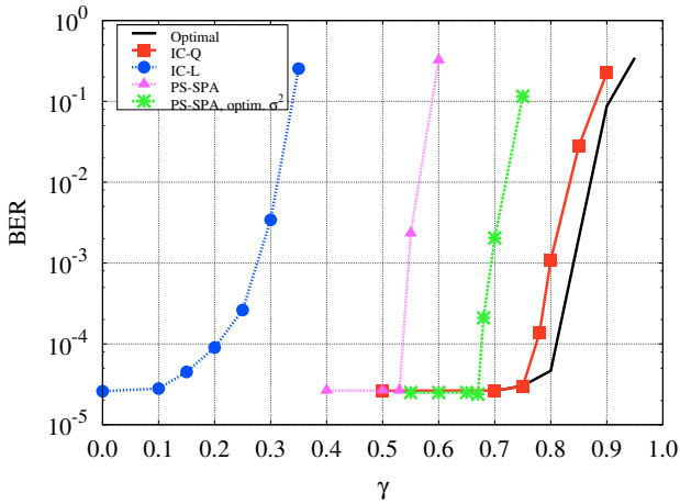
Fig. 7. CDMA system with N = 4 synchronous users and \text{SNR} = 1.35 dB. All interferers are characterized by the same value of \gamma .
