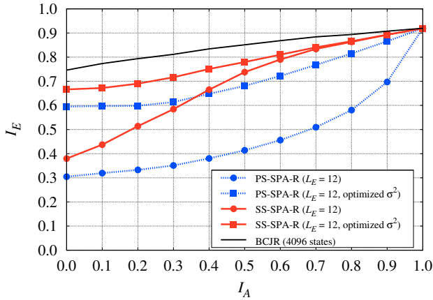
Fig. 5. EXIT charts for different algorithms over ISI channel C1, when a binary modulation is adopted and the value of the SNR is equal to 3 dB.
