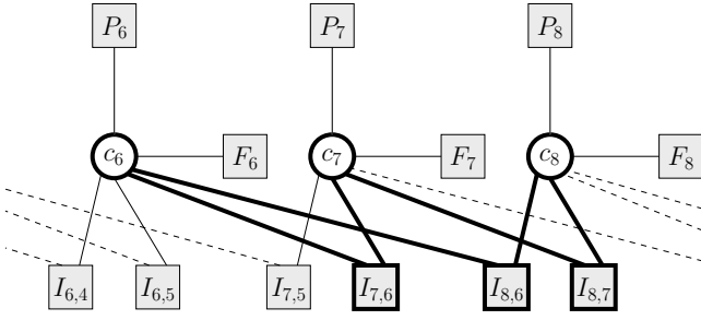
Fig. 1. Three sections of the factor graph corresponding to (12), for the case when interference between c_n and c_m arises only if |m - n| \in \{1, 2\} .
