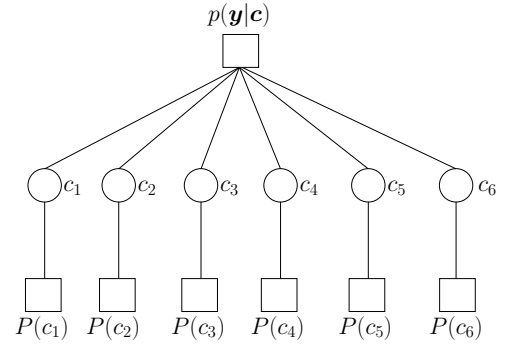
Fig. 4. Factor graph corresponding to (20).
