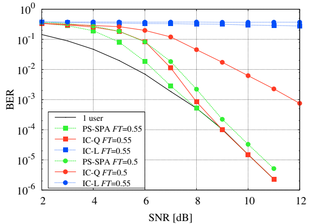
Fig. 8. FDM systems with U = 3 synchronous users. A 8-PSK and a rate 1/2 convolutional code are employed.
