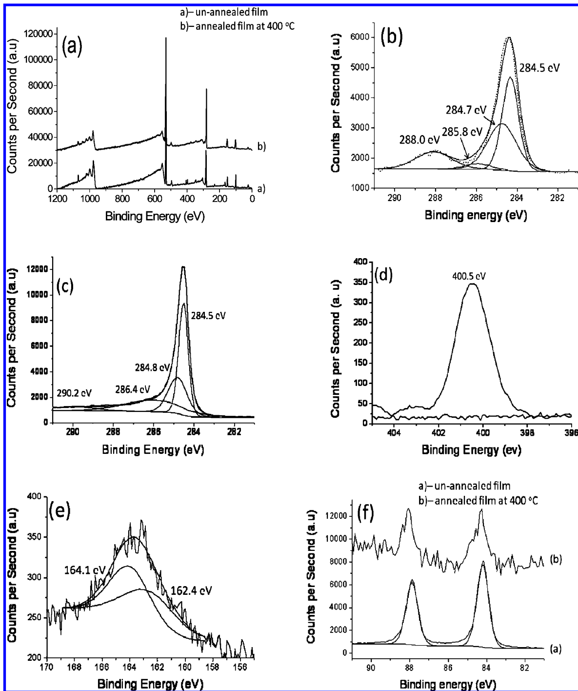
Figure 3. (a) XPS survey scan of MWCNT-Au-Cys films before and after annealing. The peaks corresponding to nitrogen and sulfur disappear after annealing. (b) Deconvoluted C 1s peak for the unannealed film. (c) Deconvoluted C 1s peak for the annealed film. (d) N 1s peak (400.5 eV) before annealing; disappears after annealing. (e) Deconvoluted S 2p peak. (f) Au 4f peaks are present both before and after annealing.
