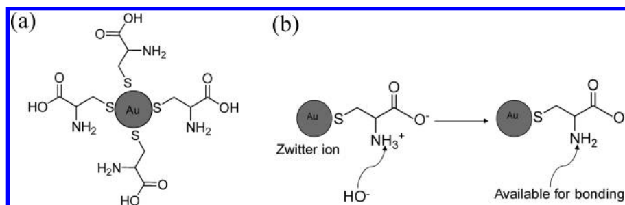
Figure 1. (a) Schematic depicting the attachment of cysteine molecules to make Au-Cys nanoparticles. (b) Schematic showing the availability of the -\text{NH}_2 group for bonding upon changing the pH by addition of base ( \text{OH}^- ) ions.
