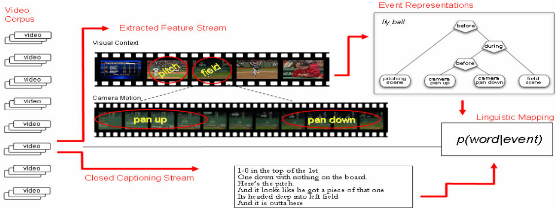
Figure 1. Video processing pipeline for learning situated models of meaning.
