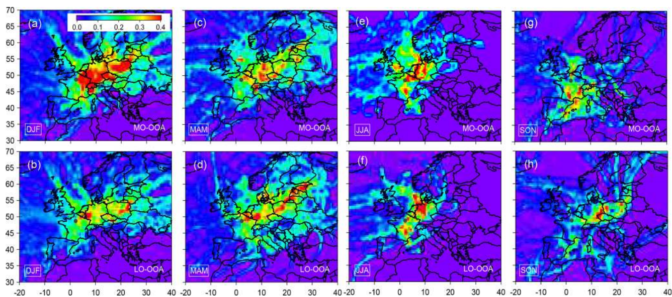
Figure 10. Maps for potential source origins of regional transport that may contribute to SOA (including MO-OOA and LO-OOA) burdens at SIRTa. Observed data points with wind speed (less than 4 \text{ m s}^{-1} ) and in the presence of precipitation events are filtered for the PSCF calculation. The solid black point in each plot represents the location of the sampling site.
