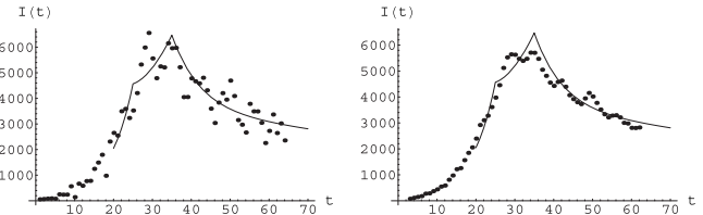
Fig. 8. Fit of epidemiological data (points) for new daily infectives, obtained by the function I(t) arising from numerical solution of the A-SIR equations; see text for parameter values and other details. Here time is measured in days, with day 0 being February 20. Left: Raw data for daily new infectives. Right: Smoothed data, smoothing corresponding to average over five days.
