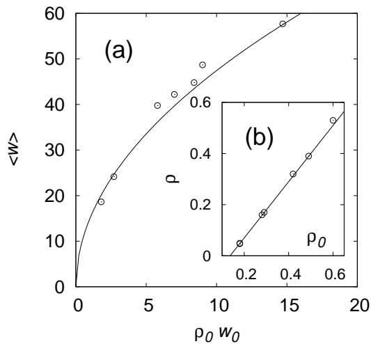
Fig. 15. (a) The average width \langle w \rangle as a function of the product between the incoming dune density \rho_0 and the width w_0 of the incoming dunes at the boundary. (b) The final stationary density \rho of the dune field as function of the initial density \rho_0 at the boundary. Note that below \rho_c (black circle) no dune field formation can be attained.
