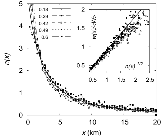
Fig. 13. Normalized local dune density n(x) \equiv N(x)(x_{\max}/dx)/N , where N(x) is the fraction of the total number of dunes N placed between x - dx and x + dx , as function of the downwind distance x for different input dune densities (symbols). The solid line corresponds to the 1/w^2(x) fit (see text). Inset: the local dune mean size w(x) scales as \langle w \rangle / \sqrt{n(x)} (solid line).
