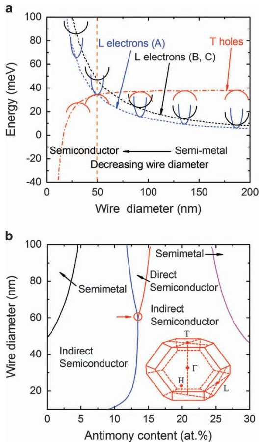
Figure 4. (a) The electronic band structure of Bi quantum wires showed the energy versus wire diameter of the highest subbands for the T -point hole carrier pocket as well as for the L -point electron carrier pockets, (b) phase horizontal diagram of the electronic band structure of \text{Bi}_{1-x}\text{Sb}_x nanowires. The centre point at the condition where the 10 hole pockets coalesce in energy. (Adapted with permission from refs 47 and 54).
