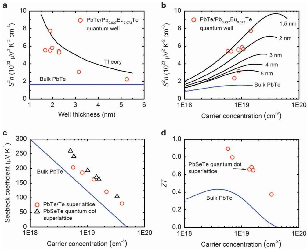
Figure 3. (a) S^2n of PbTe/Pb 0.927 Eu 0.073 Te quantum wells as a function of well thickness at 300 K, (b) S^2n of PbTe/Pb 0.927 Eu 0.073 Te quantum wells as a function of carrier concentration at 300 K, (c) Seebeck coefficient as a function of carrier concentration for n-type PbTe-based quantum wells and (d) ZT as a function of carrier concentration of n-type PbTe-based quantum wells. (Adapted with permission from refs 22 and 23).
