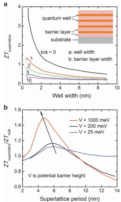
Figure 5. (a) ZT of superlattice composed of quantum wells of \text{Bi}_2\text{Te}_3 and barrier layers of \text{Pb}_{0.75}\text{Sn}_{0.25}\text{Te} as a function of ratio b/a , where a is the thickness of quantum well and b is the thickness of barrier layer, (b) figure of merit ZT of \text{Bi}_2\text{Te}_3 superlattice (scaled by ZT_{\text{bulk}} ) as a function of the superlattice period for several potential barrier heights. (Adapted with permission from refs 56 and 58).
