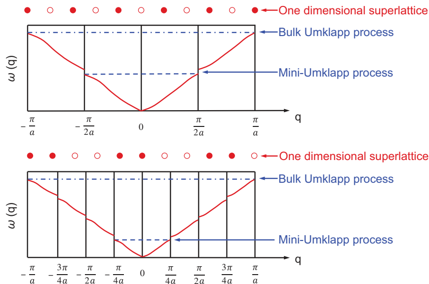
Figure 7. Brillouin zone of the superlattice, the dash-dotted lines are the bulk Umklapp process wavevectors and the dash lines are the smallest mini-Umklapp process wavevectors.
