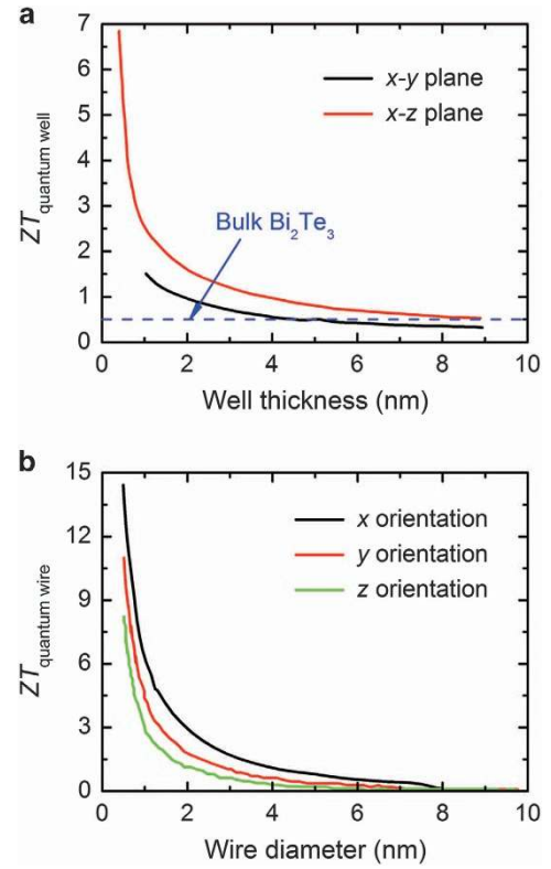
Figure 2. (a) ZT of quantum well as a function of the layer thickness, (b) ZT of quantum wire as a function of the diameter. (Adapted with permission from refs 6 and 7).
