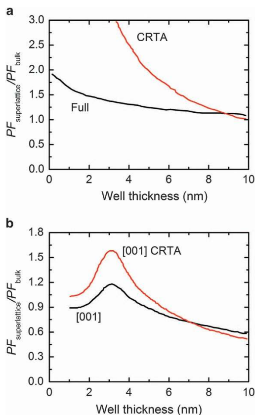
Figure 6. (a) Well-width dependence of PF for PbTe [001] quantum well superlattice with infinite barrier height scaled to corresponding bulk PF . Black solid line is full calculation and red solid line is from constant relaxation time approximation (CRTA), (b) PF for PbTe quantum superlattice grown in the [001] (black solid line) for potential offsets V = 1,000 meV, well width equal to barrier width. Red solid line is for PbTe [100] in the CRTA. (Adapted with permission from ref. 59).
