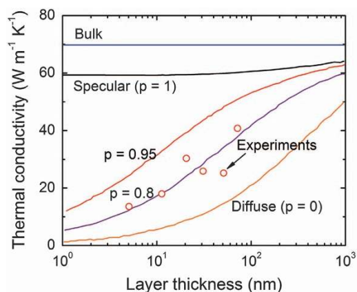
Figure 8. Thermal conductivity as a function of the layer thickness for GaAs/AlAs superlattices of equal layer thickness at room temperature.
