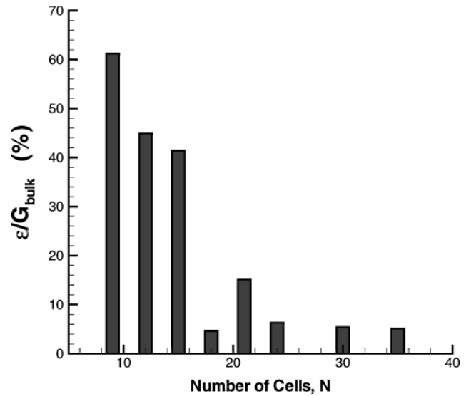
Fig. 10 Shear modulus of the subregions converges to that of the bulk sample as the size of the subregion approaches 18 mean cell diameters.
