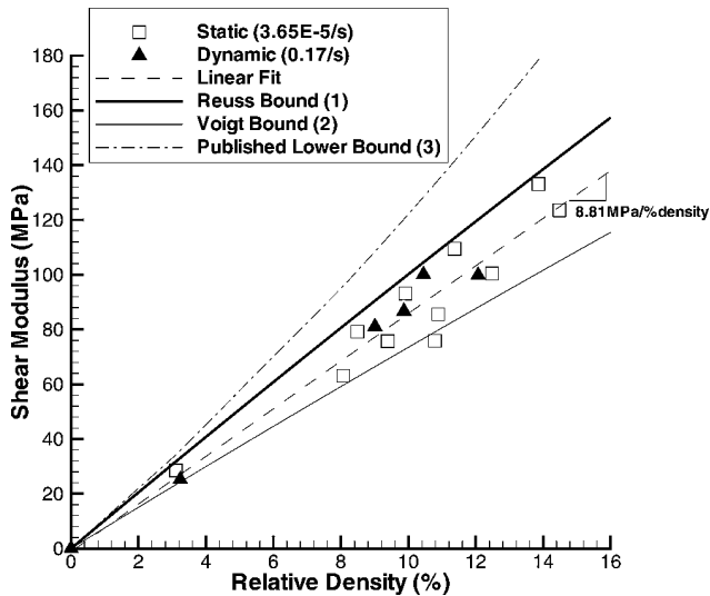
Fig. 7 Model produces appropriate bounds for the experimental shear moduli.
