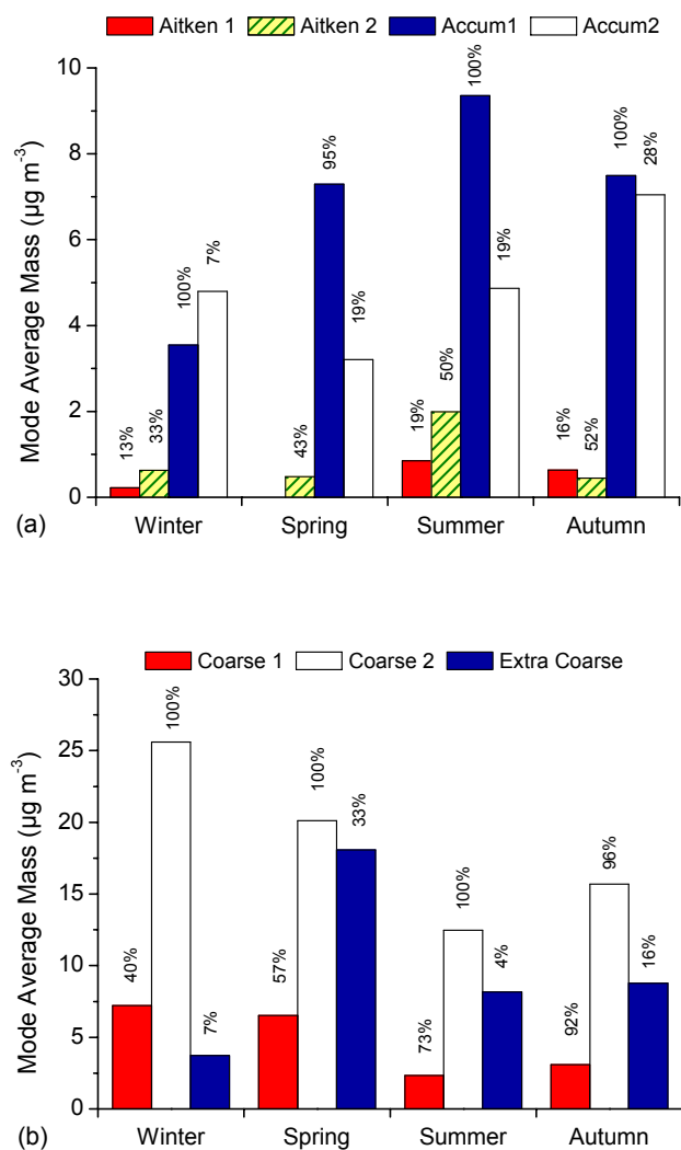
Fig. 7. Seasonal variability of the average mass of each mass mode for the period July 2004–July 2006. The modes are presented separately for the fine (a) and the coarse (b) fractions. Numbers on the top of the columns indicate the frequency of occurrence of that mode into the distributions.
