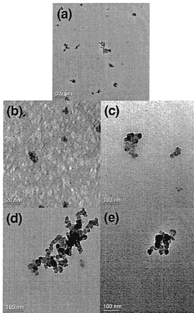
Figure 2. TEM images of soot particles generated in the ethylene diffusion flame and collected by quickly passing a carbon-film TEM grid through the tip of the flame (a–d) or by holding the grid for ~10 s in one of the vent streams (e). Panel a gives an overview of the sizes and shapes of typical soot particles, panel b shows the primary particles sizes, and panels c and e show particles in the size range of this study, while panel d shows a much larger soot agglomerate.
