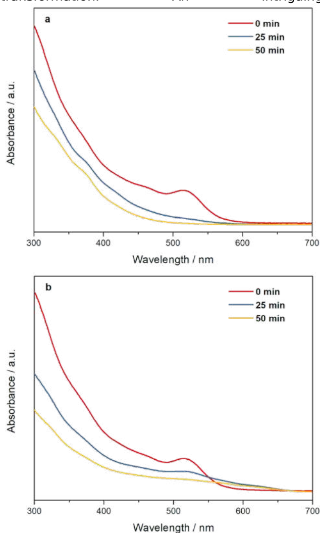
Figure 3. In situ UV-vis of \text{Au}_{22}(\text{SG})_{18} transformation with (a) 5.5eq and (b) 1eq thiol. The solution temperature was kept at 73^\circ\text{C} .
