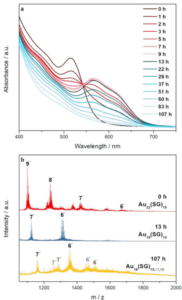
Figure 1. The in situ transformation of \text{Au}_{22}(\text{SG})_{18} upon heating at 60\text{ }^{\circ}\text{C} : (a) UV-vis and (b) ESI-MS. In the ESI spectra, the nanoclusters species have been identified and their charge has been marked above the corresponding peaks with the loss of corresponding number of \text{H}^{+} .
